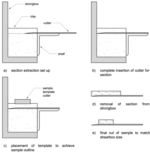
Figure 5. Sample extraction process
