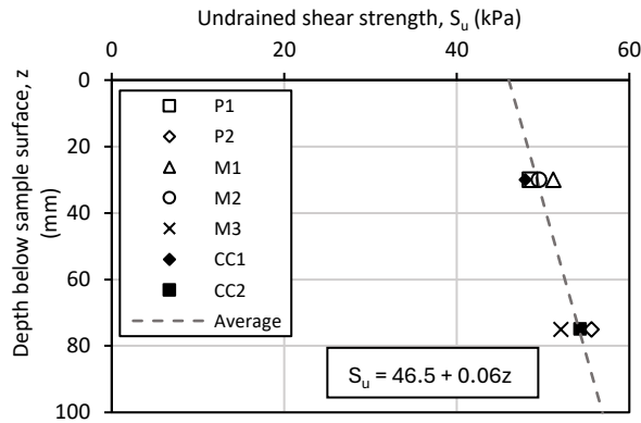
Figure 6. Undrained shear strength ( S_u ) with depth ( z ) profile calculated from water contents taken from each sample.
