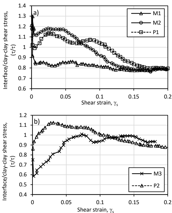
Figure 9. Normalised shear stress ( \tau/\tau ) against shear strain ( \gamma_s ) from the direct shear tests on the a) top layer, and b) bottom layer of Speswhite kaolin clay samples
