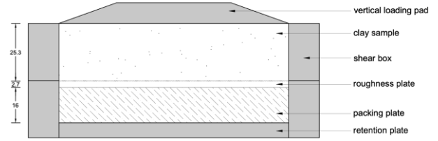
Figure 3. Cross-section of shear box for interface tests
