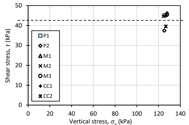
Figure 8. Shear stress ( \tau ) v. vertical stress ( \sigma_v ) results from all seven tests.
