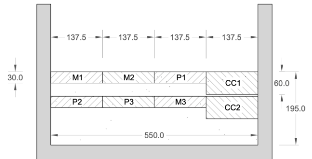
Figure 4. Schematic diagram of sample positions from consolidated clay sample
