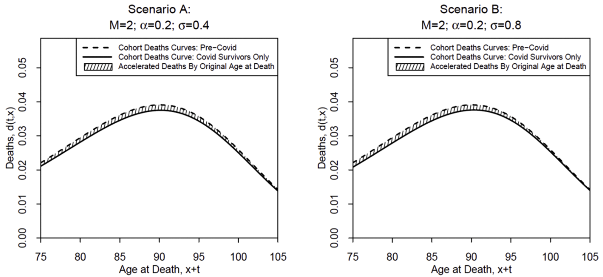
Figure 6. Deaths curves under Scenarios A and B for a cohort initially aged 75 pre-Covid (dashed curve) and post-Covid pandemic survivors only (solid curve). Hatched region: accelerated deaths.
