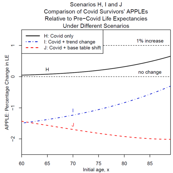
Figure 12. Impact of detrimental selection on the mean life expectancy of survivors – percentage change by initial age from the pre-pandemic life expectancy (LE) to the APPLE for Scenarios H, I, and J, which all assume M = 0.4 , \sigma = 0.8 , and \alpha = 0.8 (Equation (27)). Scenario H: Covid only. Scenario I: Covid plus a post-pandemic reduction in the assumed mortality improvement rate. Scenario J: Covid plus a post-pandemic parallel upward shift in the base mortality table. (See Equation (35).)
