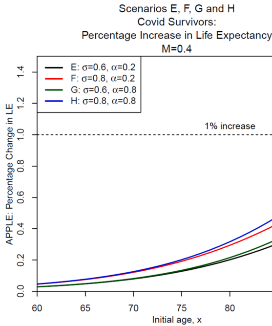
Figure 11. Impact of detrimental selection on the mean life expectancy of survivors – percentage change by initial age from the pre-pandemic life expectancy (LE) to the APPLE for Scenarios E, F, G and H (Equation (27)). The four curves show the sensitivity to changes in mortality heterogeneity in relative risk, \sigma , and proportion infected, \alpha , of the percentage change in LE in the four scenarios, when the magnitude of the pandemic M_2 = 0.4 (low, consistent with experience in England).
