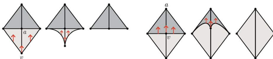
Figure 2. Strong collapse (left) vs internal strong collapse (right).
