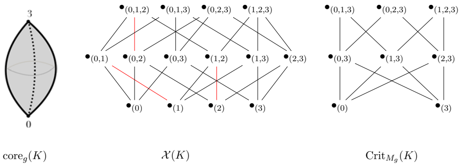
Figure 5. Left : The strong internal core associated to the map g: V(K) \rightarrow \mathbb{R} on vertices (Fig. 3). Centre : The face poset \mathcal{X}(K) , with the acyclic matching M_g induced by internal strong collapses, in red. Right : The critical poset \text{Crit}_{M_g}(K) . Here, \text{core}_g(K) has two 0-cells, three 1-cells and three 2-cells.
