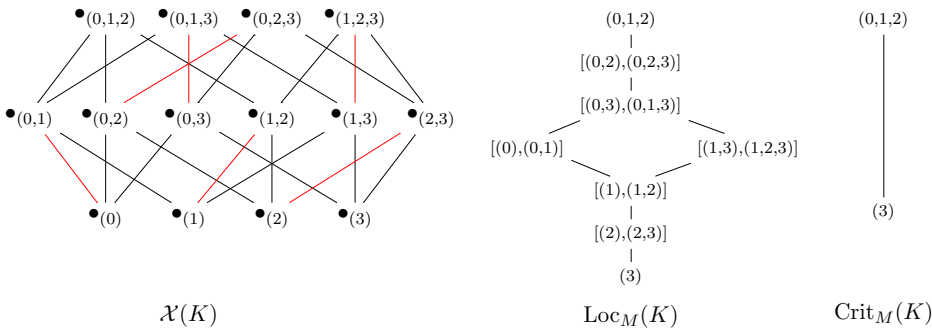
Figure 4. Left: The face poset \mathcal{X}(K) , for K the boundary of a 3-smplex, with an acyclic matching M depicted in red. Centre: The localization poset \text{Loc}_M(K) . Right: The critical poset \text{Crit}_M(K) (c.f. Fig 3).
