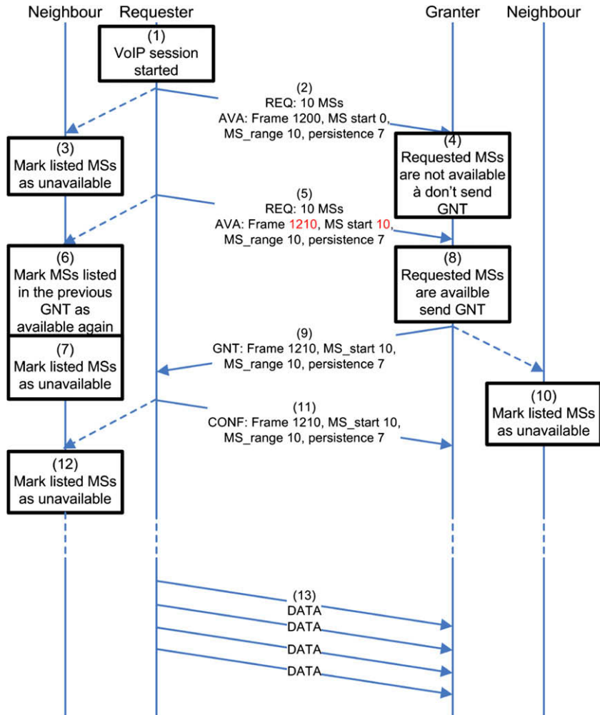
Fig. 5. Message exchange procedure for the continuous scheduler.
