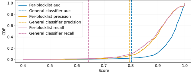
Figure 6: General vs. per blocklist classifier performance.
