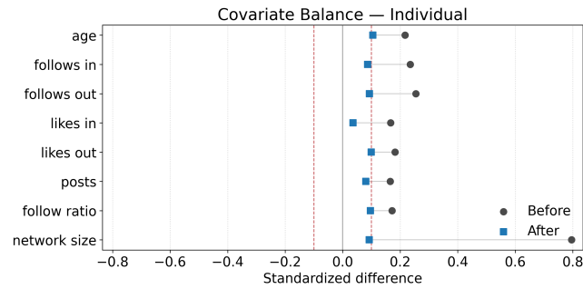
Figure 10: Covariate balance for individual blockings.
