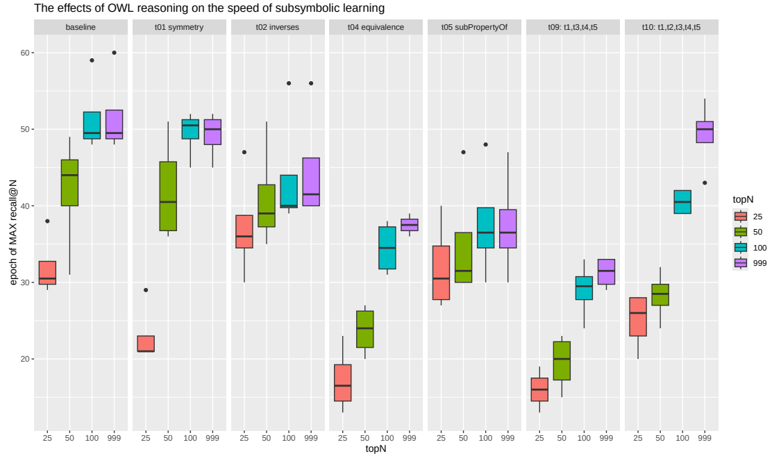
Figure 4.9: The effects of OWL reasoning on the speed of subsymbolic learning.
