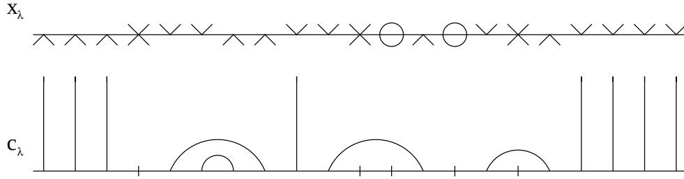
Figure 4: Another example of the cap diagram construction.
