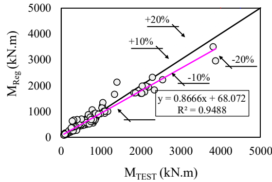
Fig. 6: Comparative analysis between the regression expression and tests
