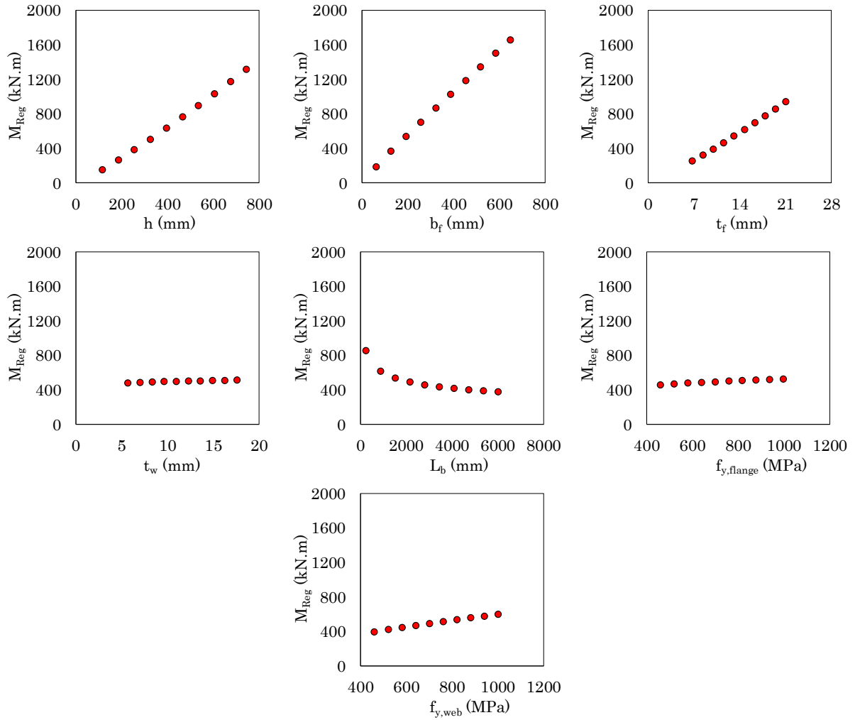
Fig. 7: The influence of the key parameters on resistance
