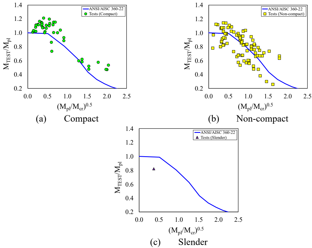
Fig. 3: ANSI/AISC 360-22 vs. tests
