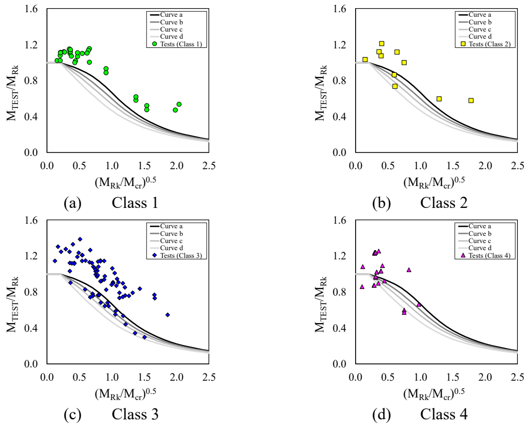
Fig. 2: BS EN 1993-1-1 General Method vs. tests
