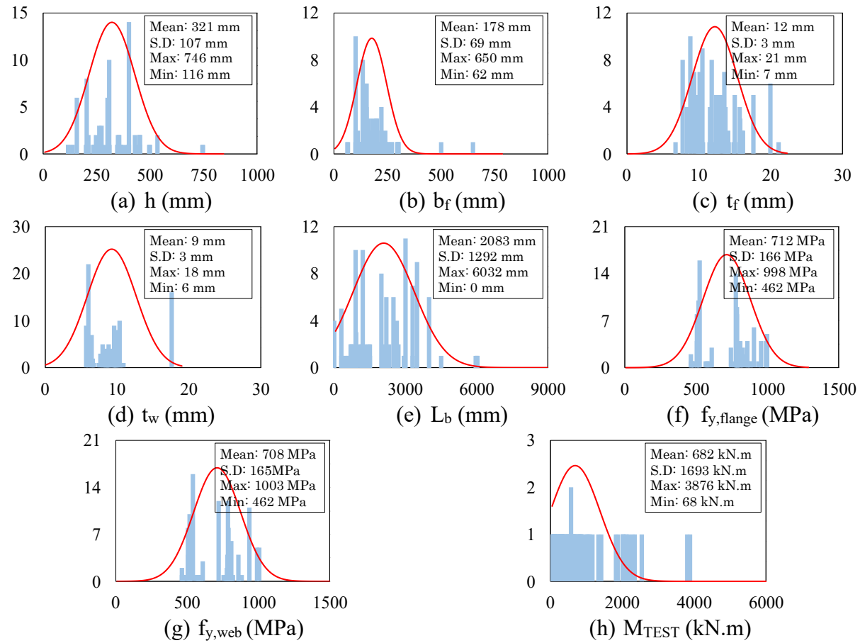
Fig. 1: Normal distribution of the database
