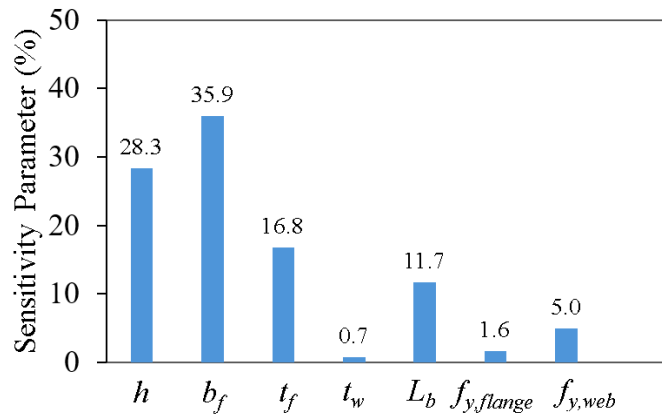
Fig. 8: The sensitivity of the key parameters on the resistance
