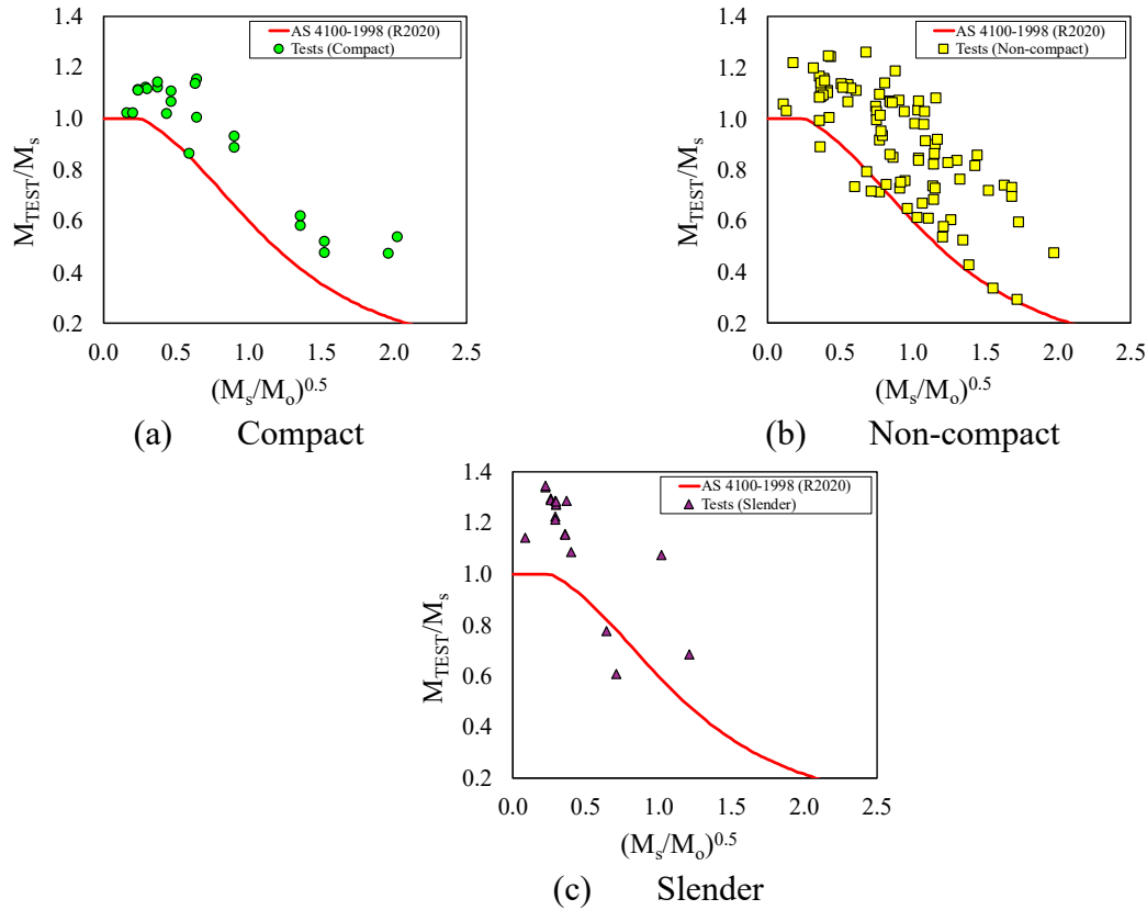
Fig. 4: AS 4100-1998 (R2020) vs. tests
