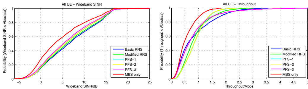
Figure 5. SLS Results for all UEs served by MBS and RNs
