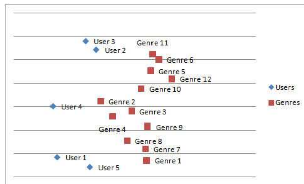
Fig. 10 SVD - Results
