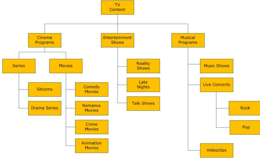
Fig. 1 AVATAR - Ontology [16]
