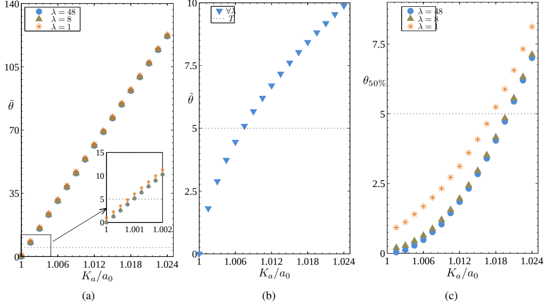
Figure 2.2: The characteristics of the most common time-to-fill of sell limit orders submitted at different prices K_a \geq a_0 : (a) the average time-to-fill, (b) the mode time-to-fill, (c) the median time-to-fill. Results are shown for parameters in Table 2.2.
