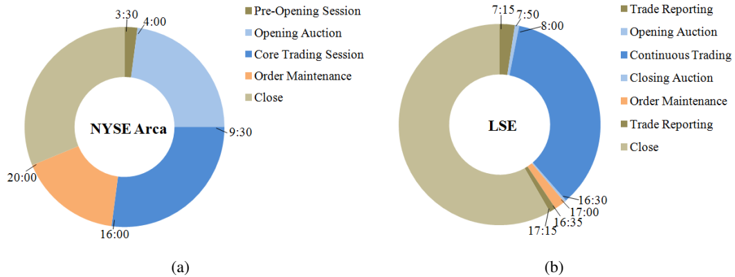
Figure 1.2: Market phases on a regular trading day (a) on the New York Stock Exchange Arca (NYSE Arca), and (b) on the London Stock Exchange (LSE).
