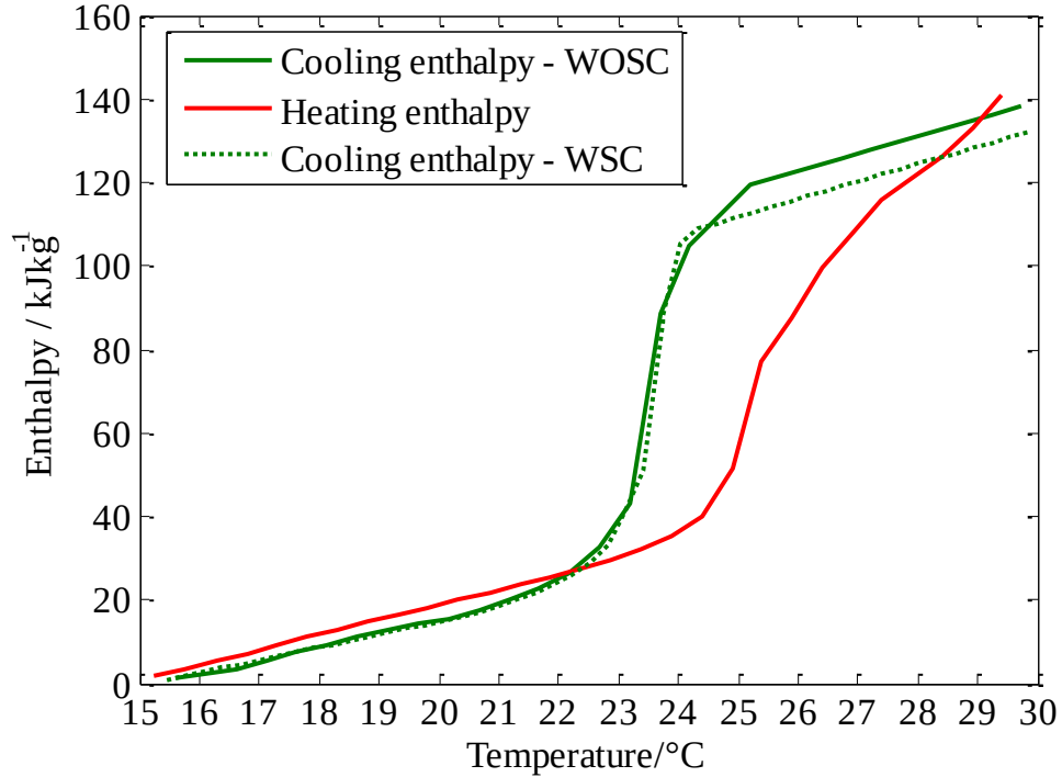
Figure 9.9: Enthalpy-temperature curves upon cooling and heating obtained from the re-evaluation of PT27 with the normalised enthalpy value of 0 \text{ kJkg}^{-1} at 15^\circ\text{C} (Cooling enthalpy WOSC – enthalpy curve upon cooling in the case when subcooling is neglected, Heating enthalpy – enthalpy curve upon heating, Cooling enthalpy WSC – enthalpy curve upon cooling in the case when subcooling is taken into account).
