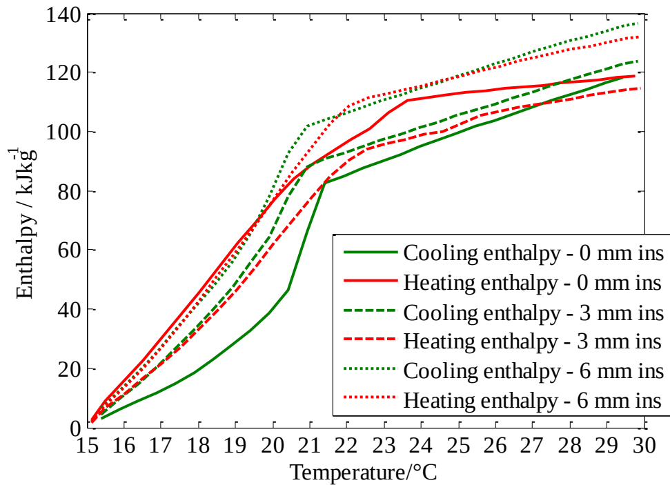
Figure 8.9: Enthalpy-temperature curves upon cooling and heating from RT21 T-history studies with various insulation thicknesses (0, 3, and 6 mm) with the normalised enthalpy value of 0 kJkg -1 at 15 °C.
