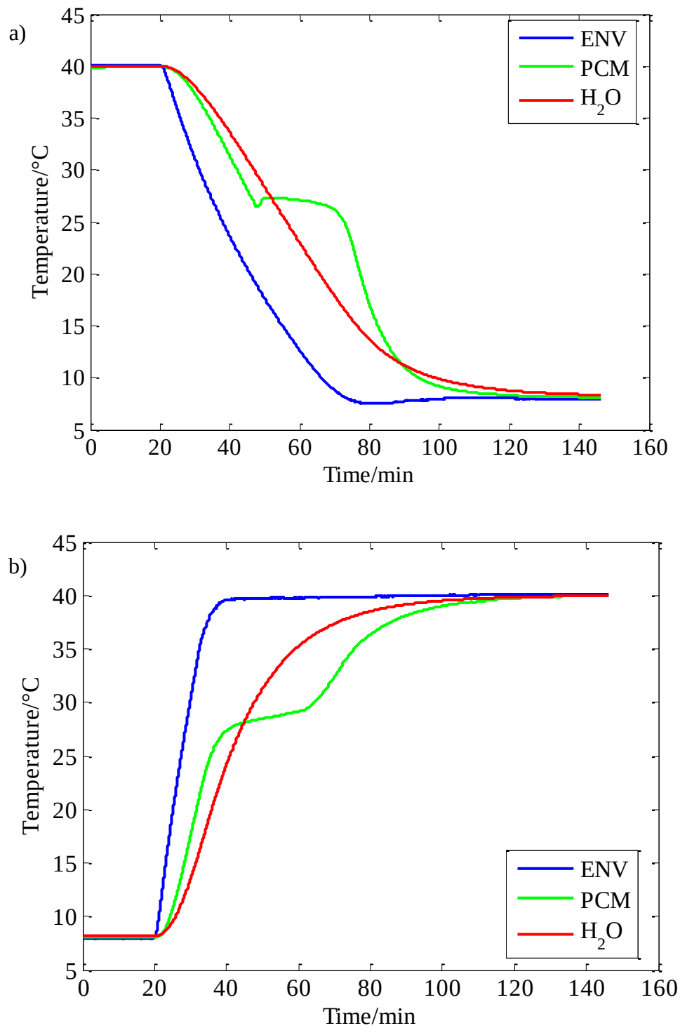
Figure 8.26: Cooling (a) and heating (b) cycles in the advanced T-history characterisation of PT28 (ENV – environmental temperature, PCM – temperature of the PCM sample, H 2 O – temperature of the reference sample).
