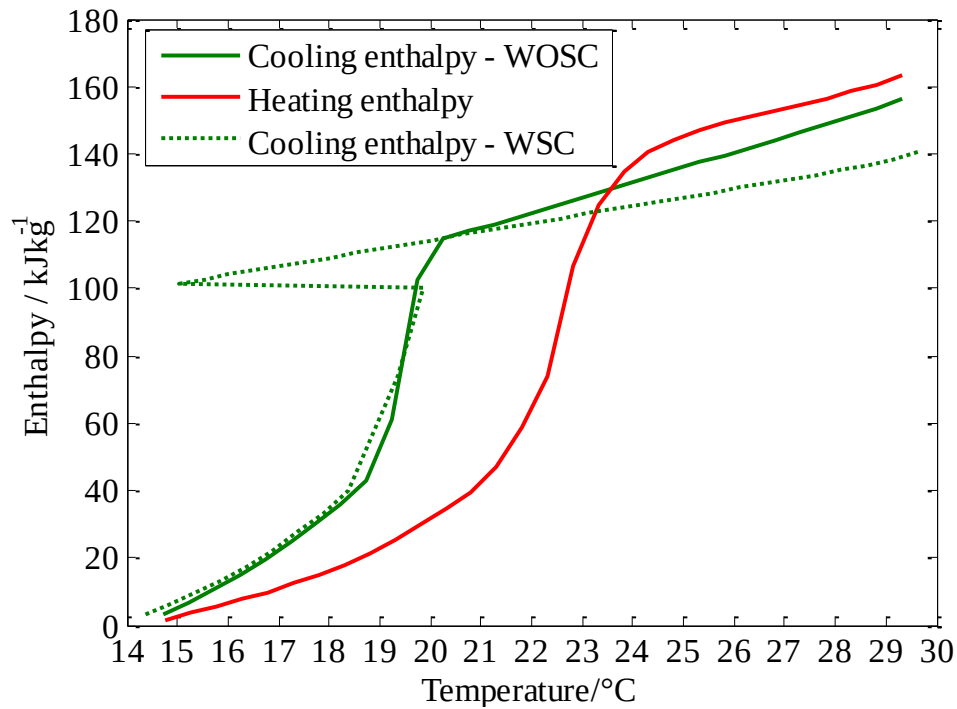
Figure 9.4: Enthalpy-temperature curves upon cooling and heating obtained from the advanced T-history characterisation of SP22 with the normalised enthalpy value of 0 \text{ kJkg}^{-1} at 15^\circ\text{C} (Cooling enthalpy WOSC – enthalpy curve upon cooling in the case when subcooling is neglected, Heating enthalpy – enthalpy curve upon heating, Cooling enthalpy WSC – enthalpy curve upon cooling in the case when subcooling is taken into account).
