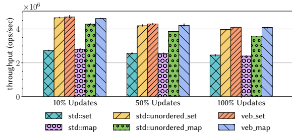
Figure 12. Single-threaded performance compared with C++ standard containers.
