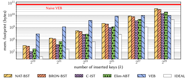
Figure 11. Memory footprint (bytes). Log-scaled y-axis.
