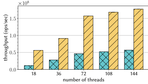
(a) Performance. 50% update workload. u = 2^{28} .
