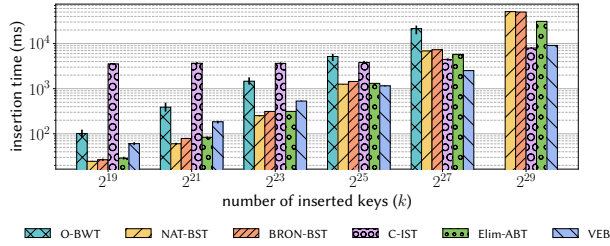
Figure 9. Insertion time (ms). Log-scaled y-axis.
