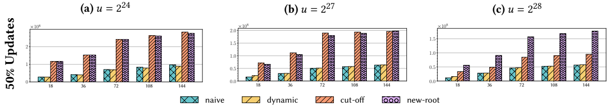
Figure 6. Throughput comparison of our vEB sets. \frac{u}{2} keys are inserted before measurements. x-axes: number of threads.
