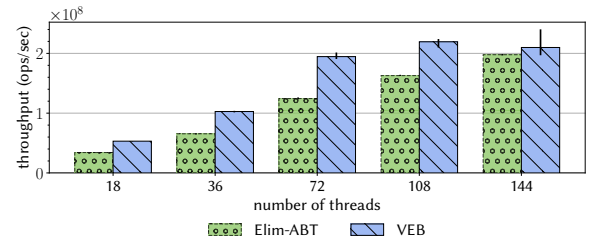
Figure 13. Successor operation performance. Elim-ABT is non-linearizable.
