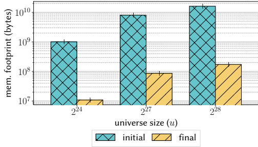
(b) Memory usage for \frac{u}{2} keys. Log-scaled y-axis.
