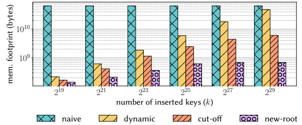
Figure 10. Memory footprint (bytes). Log-scaled y-axis.
