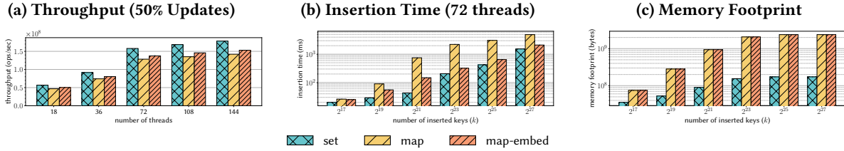
Figure 7. From vEB set to vEB map. y-axes for insertion time and memory footprint are log-scaled .
