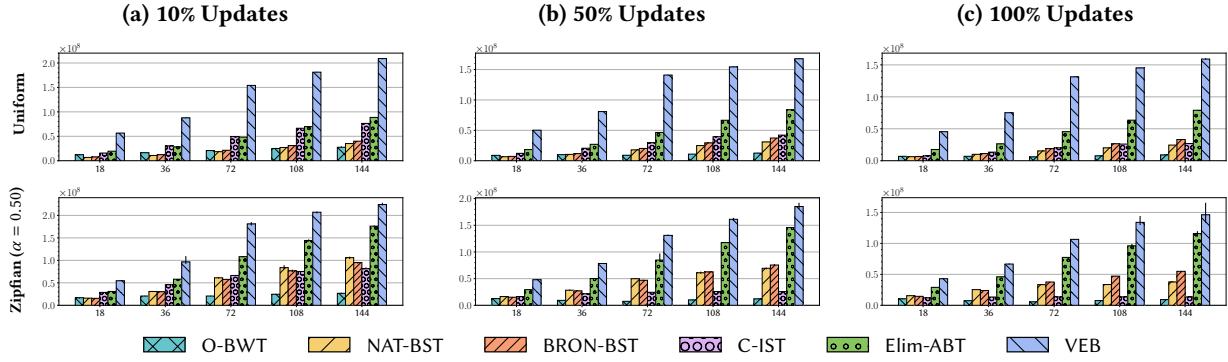
Figure 8. Performance. u = 2^{28} . \frac{u}{2} keys inserted before the measurements. x-axes: number of threads. y-axes: throughput.
