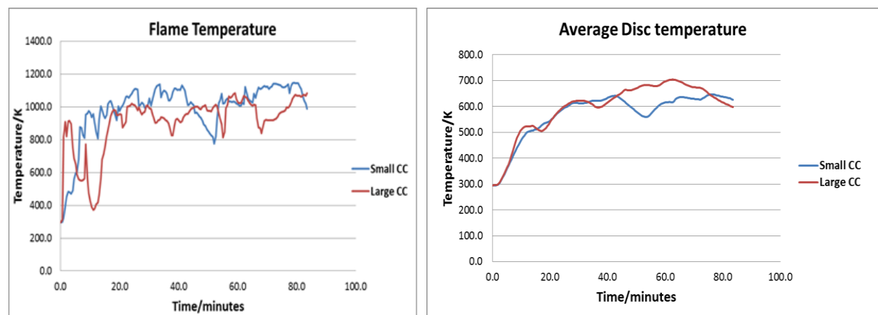
Figure 4. Comparison of temperatures achieved with large and small CCs (Note wood burn rate for large CC of 2.5 kg/hr and small CC 1.5 kg/hr)
