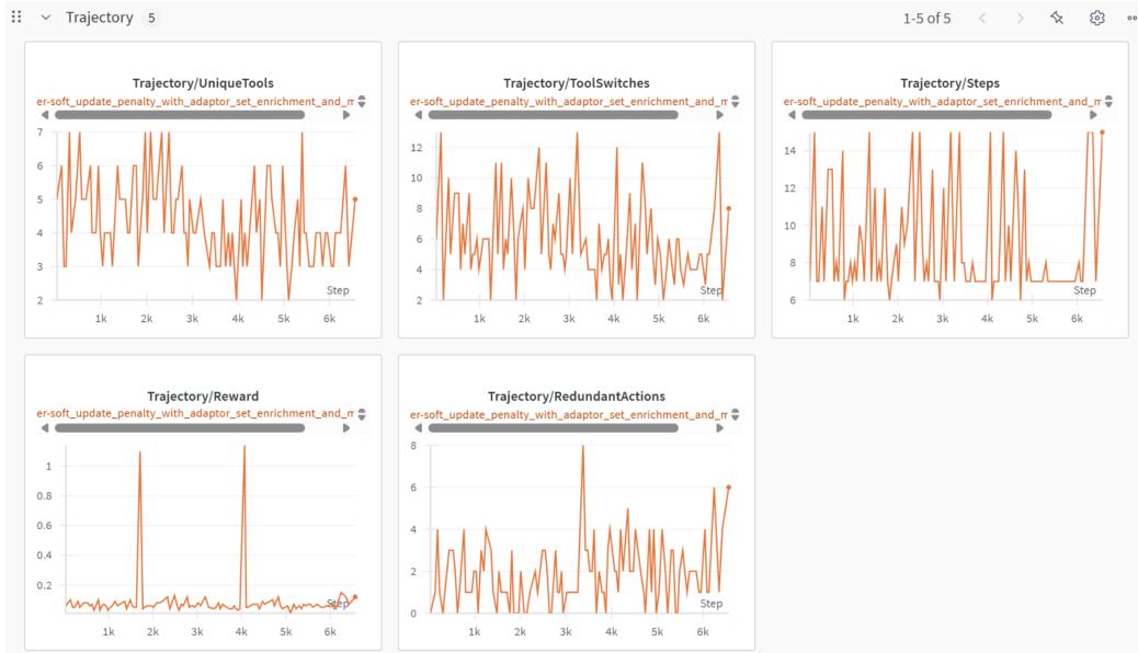
Figure 54: Trajectory-level statistics during training: unique tools, tool switches, steps per episode, reward progression, and redundant actions.
