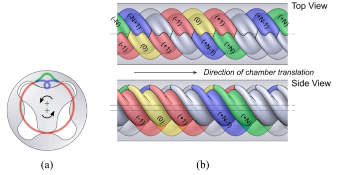
Fig. 5. Illustration of leakage paths in an internally geared screw machine (third-angle projection). (a) rotor rotation and chamber positions; (b) top and side views of chamber indexing along the axial direction. Leakage may occur between adjacent chambers as they translate during operation.
