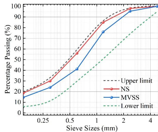
Fig. 2. Gradation curve of sand.
