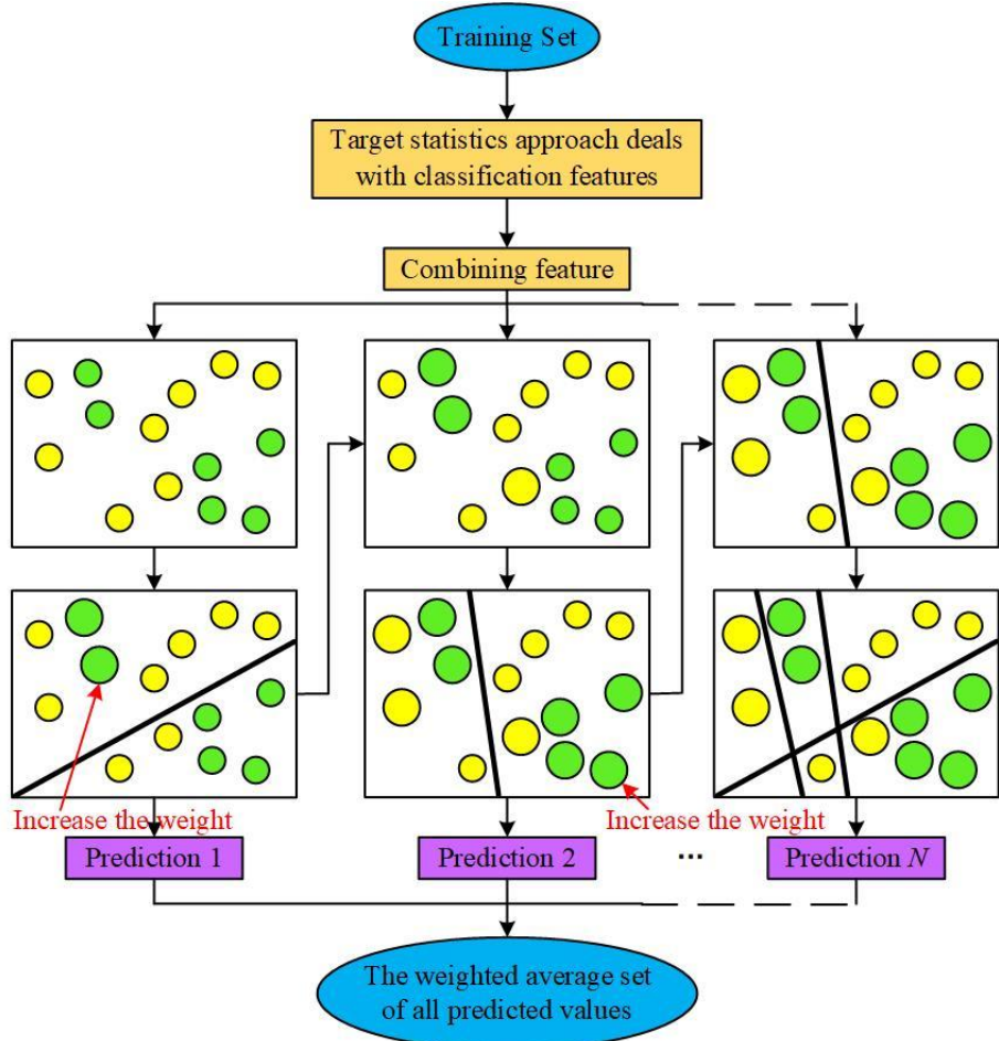
Fig. 12. CatBoost structure.
