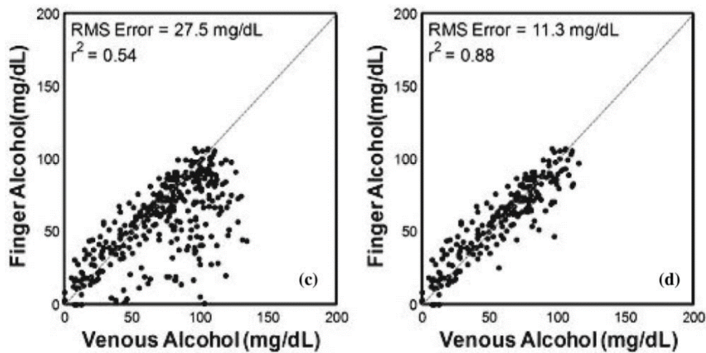
Figure 3.7: TruTouch Forearm vs Blood Ethanol Levels[10]
