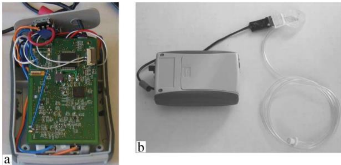
Figure 3.3: ISF alcohol sensor prototype (a: The electronic circuit use for control of the system and responsible for the measurement of ISF. b: The fully assembled system with an ISF extraction tube.
