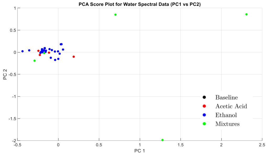
Figure 7.10: PCA scores plot for porcine skin data
