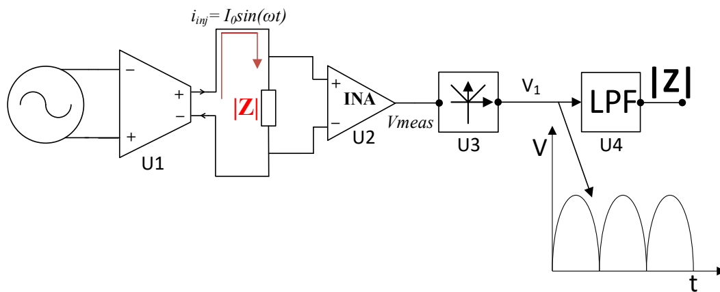
Figure 4.5: Circuit Diagram of the Impedance Measuring Module
