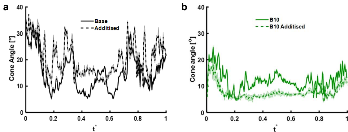
Figure 4.28: Comparison of spray cone angles for Spray C at 1 bar ambient condition.
