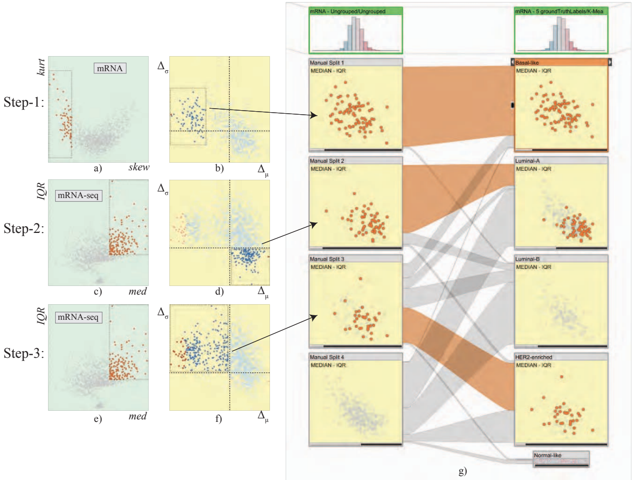
Fig. 6. Manual clustering of unstratified mRNA dataset using dual analysis views. Negatively skewed genes are selected through skew vs. kurt visualization (a) and the difference plot for the samples is updated automatically (b) where we observe a group of samples with lower values and mark them as our first cluster (b). We then switch to the mRNA-seq dataset and select genes that are higher-expressed with a large variety within the values (c,e). We identify two groups and mark them as clusters 2 (d) and 3 (f). For validation, we compare our stratification with the subtypes from the reference study and observe a significant overlap with the subtypes.
