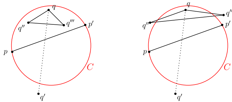
■ Figure 4 Proof of Lemma 23. The left example is in case (i); the right example is in case (ii).
