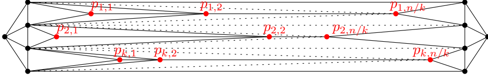
■ Figure 2 Merging k x -sorted lists \langle p_{1,1}, \dots, p_{1,n/k} \rangle, \dots, \langle p_{k,1}, \dots, p_{k,n/k} \rangle reduces to computing the Delaunay triangulation of the O(n) vertices of the triangulation shown (assuming a rescaling to compress the y -coordinates). This triangulation has D_{\text{local}} = \Theta(k) non-locally-Delaunay edges shown in dotted lines.
