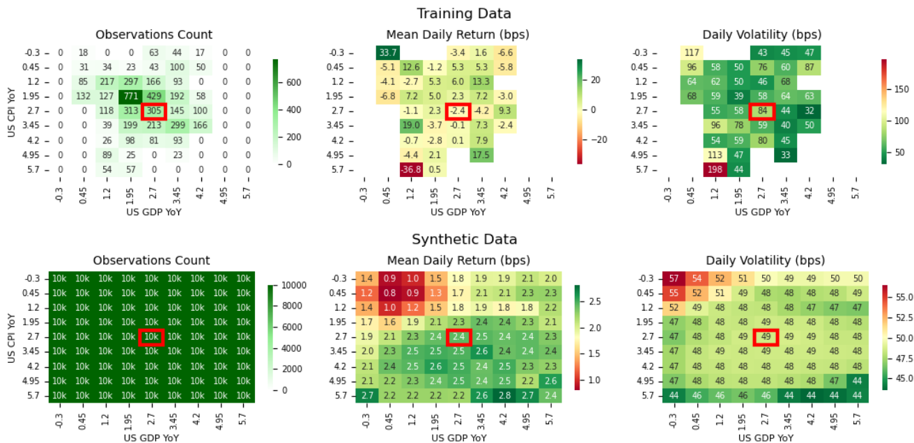
Figure 3: Macro-conditional scenario grid for an equally weighted portfolio of 16 futures contracts, conditioning on US CPI YoY (vertical) and US GDP YoY (horizontal). Top row: empirical results from training data (through 2024), showing observation counts, mean daily returns, and volatility (basis points) per macro configuration. Bottom row: MacroVAE-generated results using 10,000 simulations per cell. Red squares indicate current macroeconomic conditions. The synthetic surfaces provide smooth, complete coverage across the grid, including scenarios that are sparsely or never observed in the historical data.
