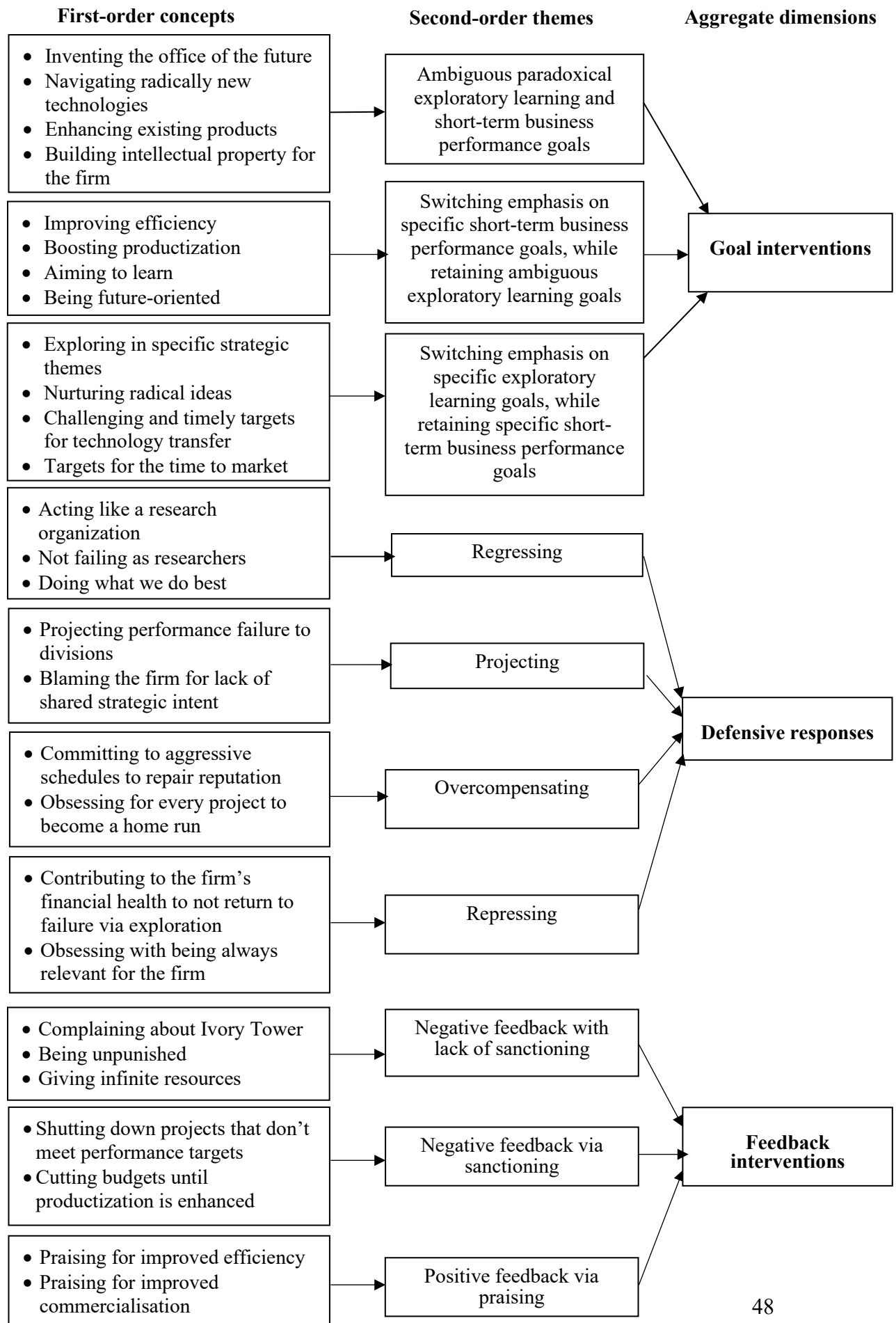
Figure 1. Data Structure
