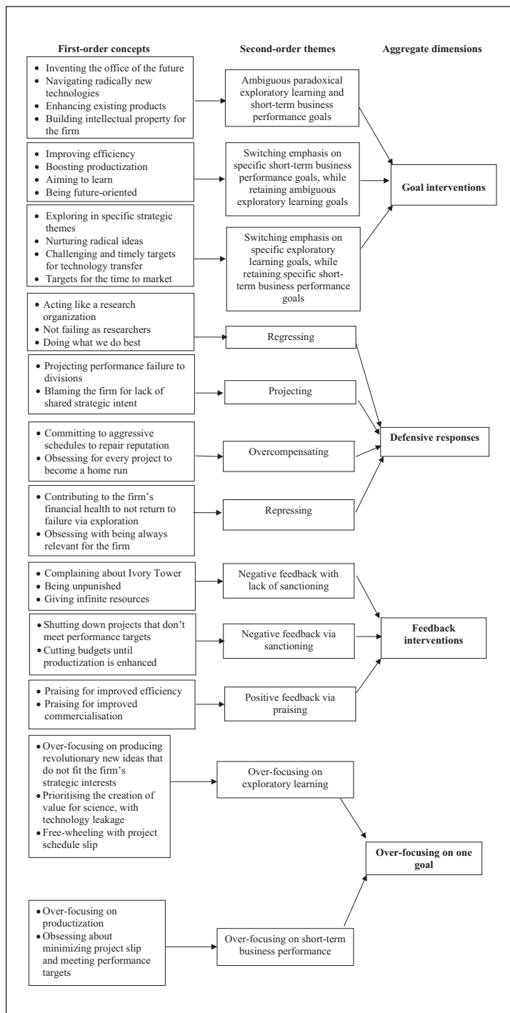
Figure 1. Data structure.
