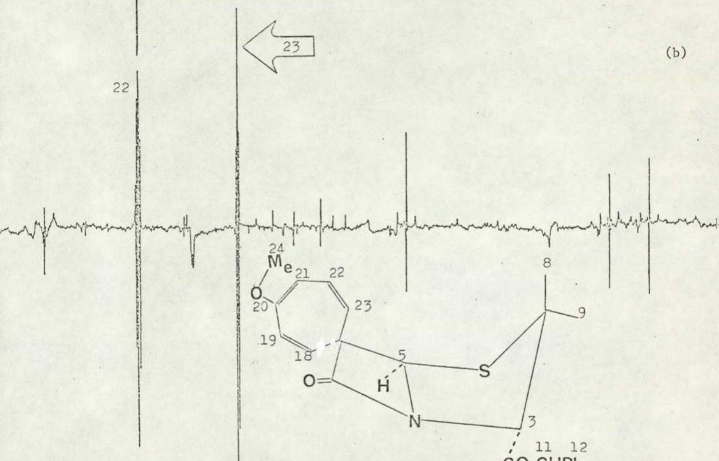
Figure 3. Partial 400 MHz spectra of (64) in \text{CDCl}_3 . (a) Normal spectrum, (b) decoupling-difference spectrum with irradiation of \text{C}_{23}\text{-H} , (c) decoupling-difference spectrum with irradiation of \text{C}_{22}\text{-H} .
