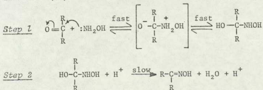
Scheme 14
