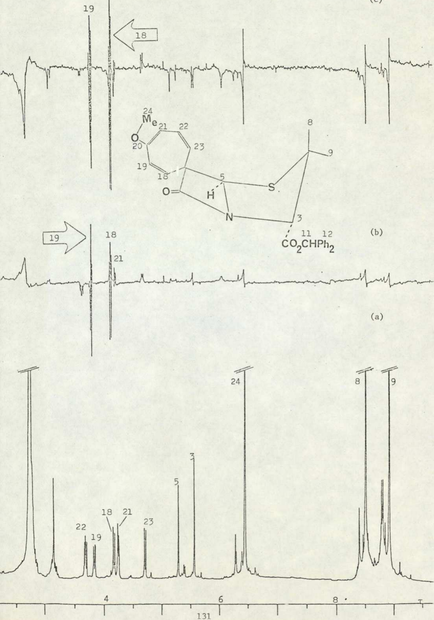
Figure 1. Partial 400 MHz spectra of ( 64 ) in \text{CDCl}_3 . (a) Normal spectrum, (b) decoupling-difference spectrum with irradiation of \text{C}_{19}\text{-H} , (c) decoupling-difference spectrum with irradiation of \text{C}_{18}\text{-H} .
