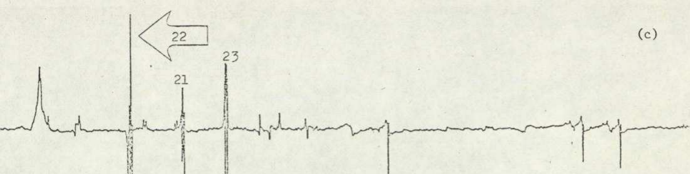
Figure 3. Partial 400 MHz spectra of (64) in \text{CDCl}_3 . (a) Normal spectrum, (b) decoupling-difference spectrum with irradiation of \text{C}_{23}\text{-H} , (c) decoupling-difference spectrum with irradiation of \text{C}_{22}\text{-H} .
