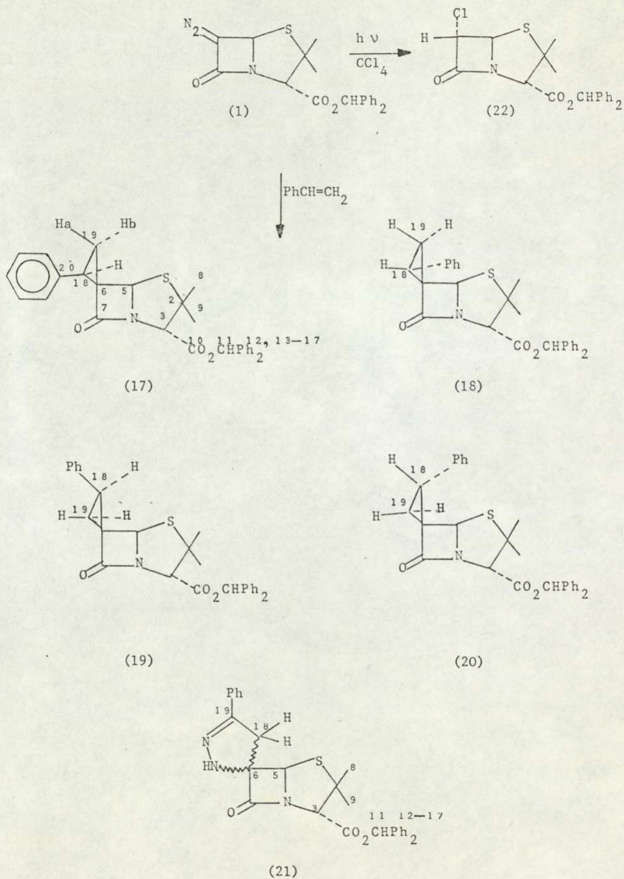
Scheme 10.
