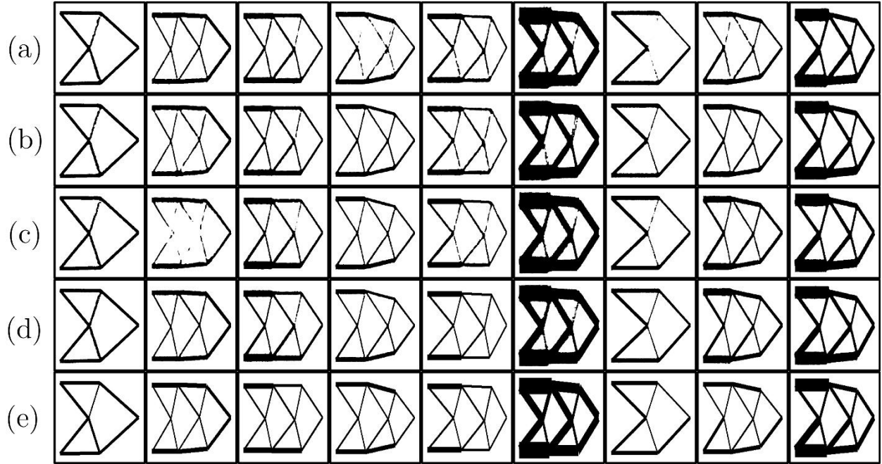
Figure 3 - Visual comparison of predictions on unseen data: (a) CNNC512, (b) FFNN64+CNN512, (c) CNN64+CNN256, (d) CNN64+CNN512, (e) ground truth for the cantilever dataset
