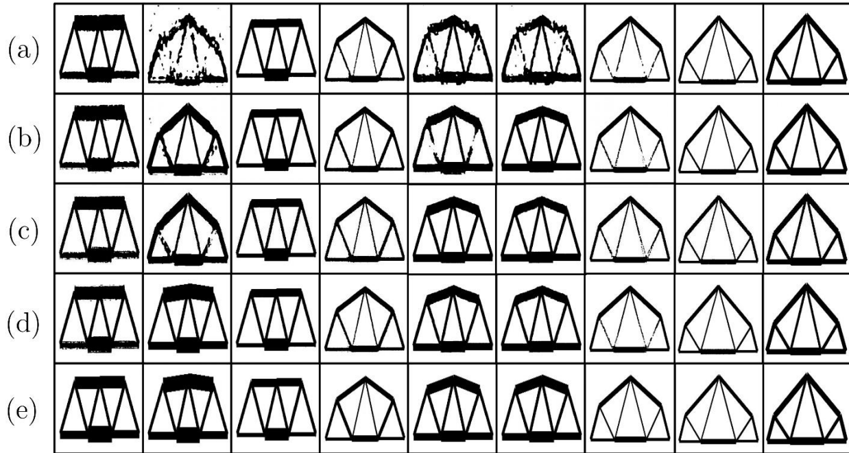
Figure 11 - Visual comparison of predictions on unseen data: (a) CNNC512, (b) FFNN64+CNN512, (c) CNN64+CNN256, (d) CNN64+CNN512, (e) ground truth for the simply supported dataset
