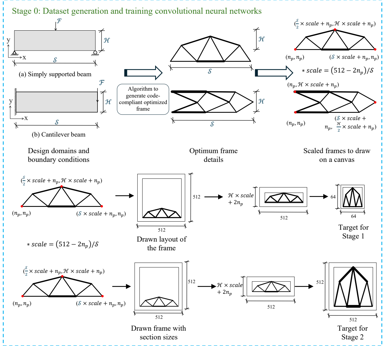
Figure 1: Data generation workflow for Stage 1 and Stage 2 CNN models
