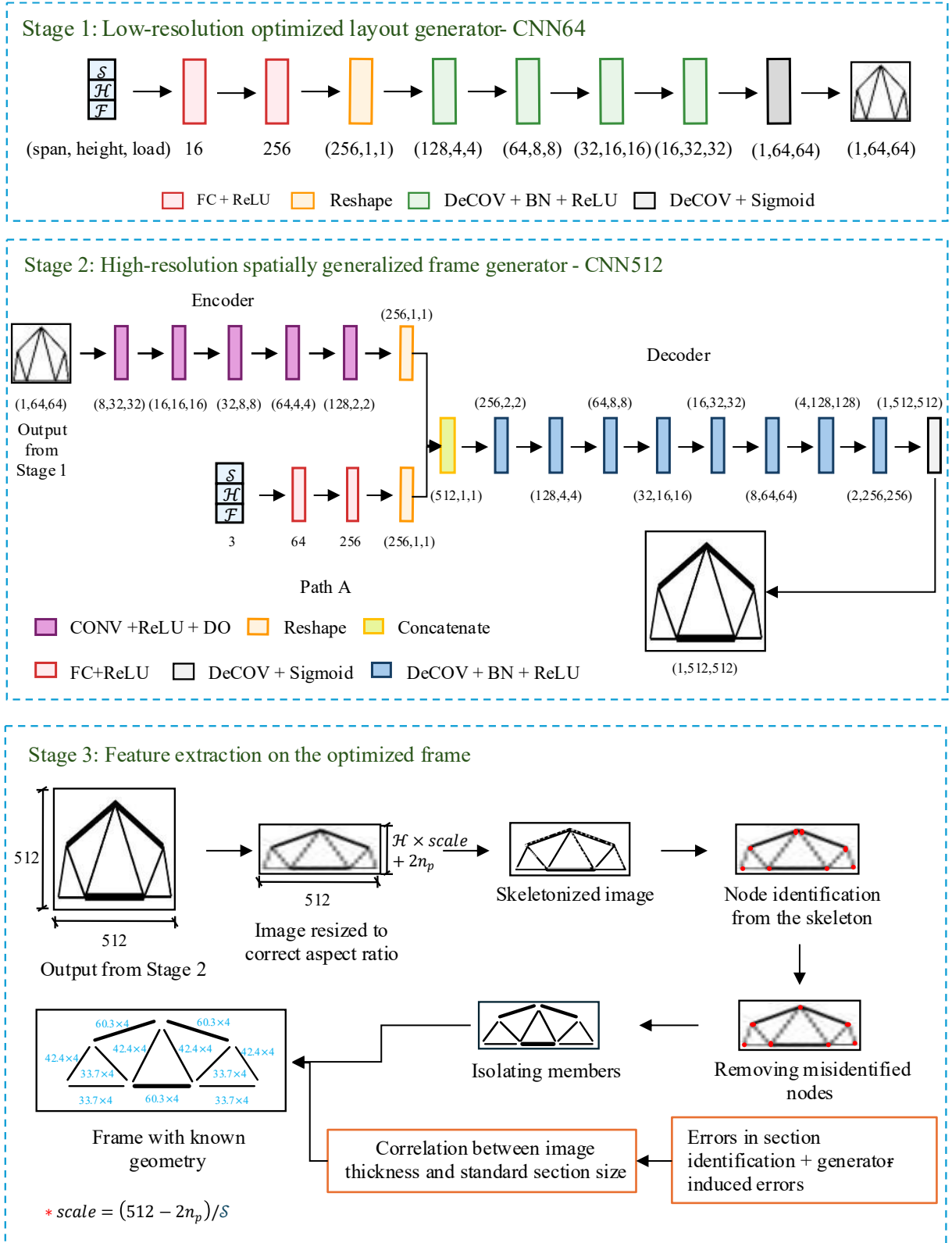
Figure 2 - Three-stage proposed workflow for generative design of code-compliant optimized frames
