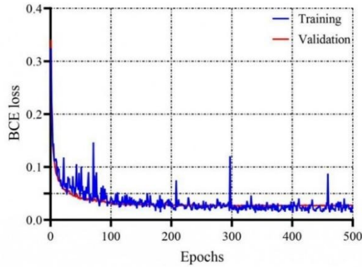
(c) Stage 1: CNN64 for simply supported dataset
