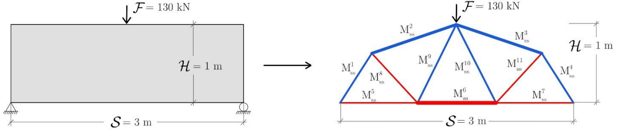
Figure 12 - Topology-size-layout optimal structure and its member identifiers for the simply supported problem with S=3 m, H=1 m, F=130 kN
