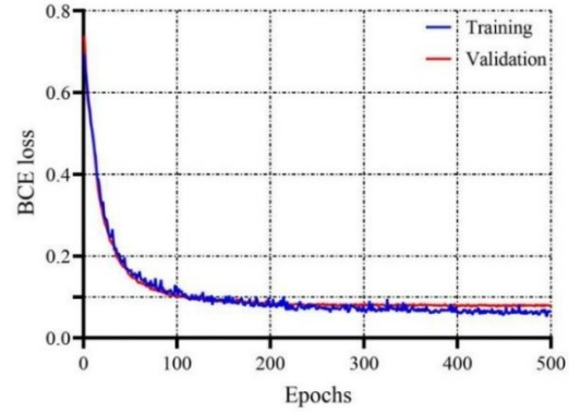
(b) Stage 2: CNN512 for cantilever dataset
