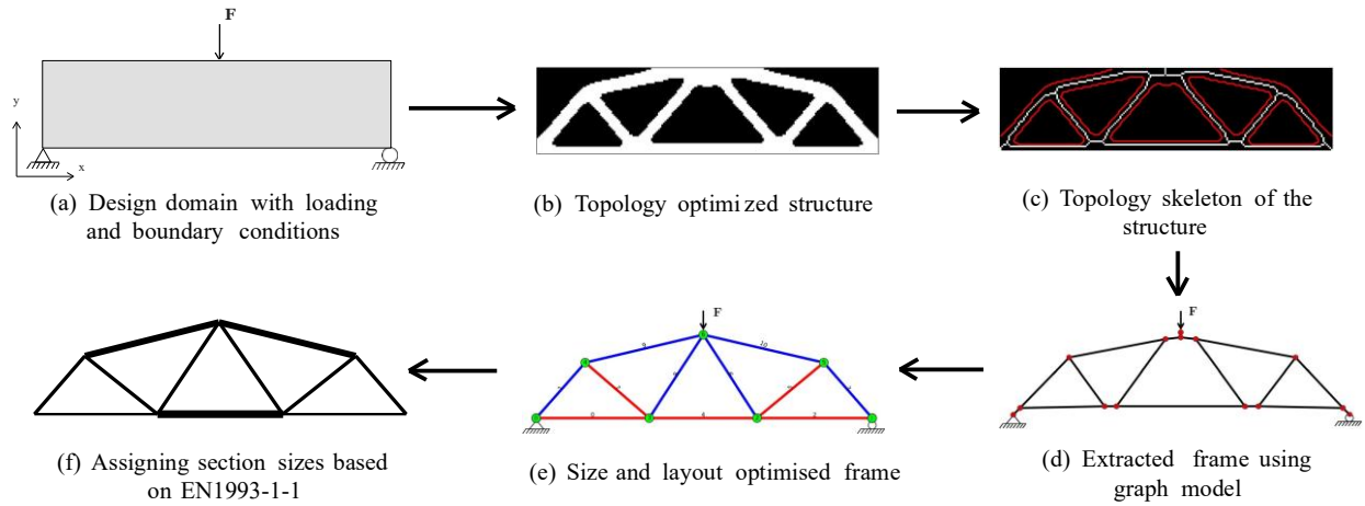
Figure 5 - Workflow for design-informed structural optimisation of 2D skeletal frames
