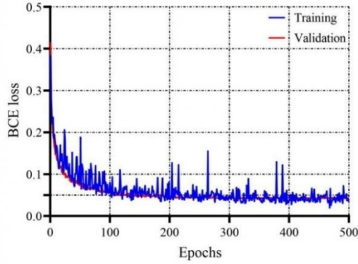
(a) Stage 1: CNN64 for cantilever dataset
