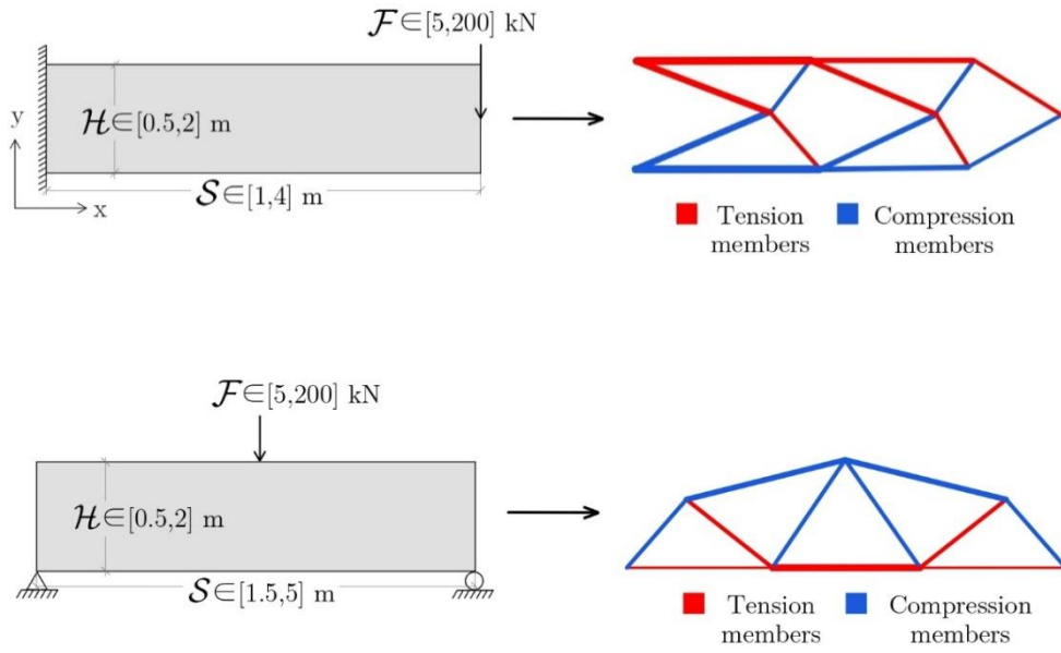
Figure 6 - Range of design variables for the (top) cantilever problem dataset (bottom) simply supported problem dataset
