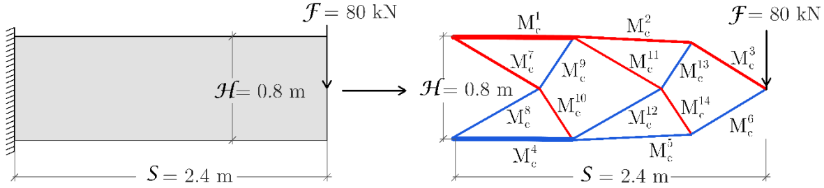
Figure 10 - Topology-size-layout optimal structure and its member identifiers for the cantilever problem with S = 2.4 m, H = 0.8 m, and F = 80 kN
