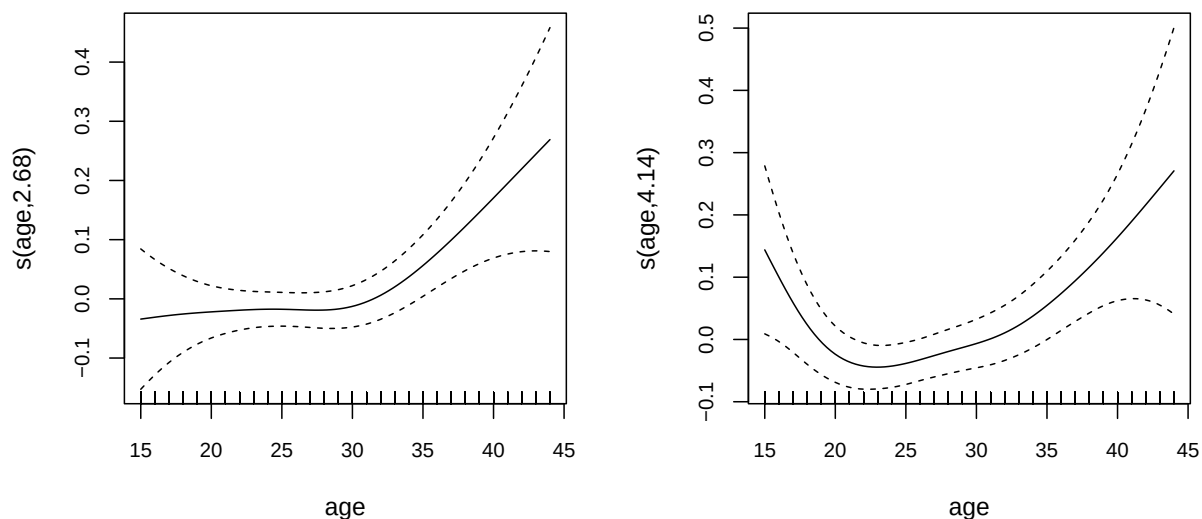
Figure 2: Estimated smooth effects of age on the predictor scales of \mu_1 (left) and \mu_2 (right), based on a Gaussian copula distributional regression model with probit margins fitted to the infant data. The y-axes show the contributions of the smooths of age to lbw and ptb , with 95% intervals. Numbers in parentheses in the smooth labels (e.g., s(\text{age}, 2.68) ) indicate the estimated degrees of freedom, reflecting the smooth's flexibility: higher values correspond to more flexible fits.
