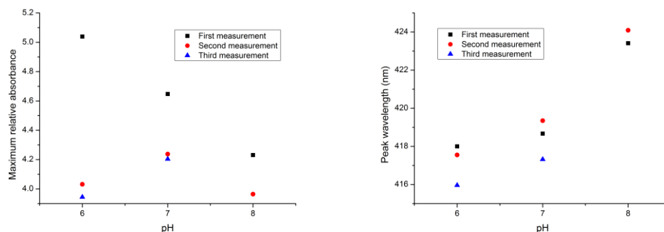
Figure 2 The maximum value of the relative absorbance (left) and the peak wavelength (right) versus pH for the consecutive measurements of the pH solutions for (PAH/BY) 8 on the glass slide. No heat treatment or drying was used in the process. (The sample is designated GS01)
