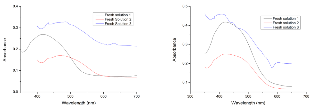
Figure 14 The spectra for the coated glass slides with (PAH/BY) 6 dipped into the fresh buffer solution for three times and each time for 60 minutes. Left: pH 6 (The sample designated GS11), Right: pH 8 (The sample is designated GS12). The samples were cured at 120°C for 4 hours.
