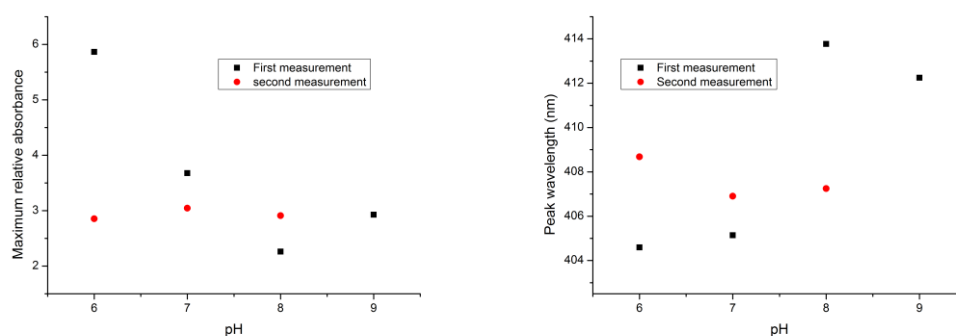
Figure 7 The maximum value of the relative absorbance (left) and the peak wavelength (right) versus pH for the consecutive measurements of the pH solutions for (\text{PAH/BY})_6(\text{PAH/SiO}_2)_2 on the glass slide. The sample was cured at 130^\circ\text{C} for 7 hours and exposed to UV light for 20 minutes. (The sample designated as GS06)
