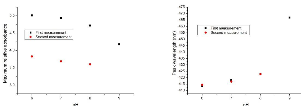
Figure 6 The maximum value of the relative absorbance (left) and the peak wavelength (right) versus pH for the consecutive measurements of the pH solutions for (\text{PAH/BY})_6(\text{PAH/SiO}_2)_2 on the glass slide. The sample was cured at 130^\circ\text{C} for 7 hours. (The sample designated as GS05)
