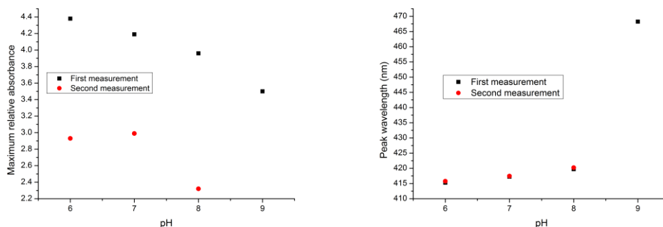
Figure 5 The maximum value of the relative absorbance (left) and the peak wavelength (right) versus pH for the consecutive measurements of the pH solutions for (\text{PAH/BY})_6(\text{PAH/SiO}_2)_2 on the glass slide. (The sample designated as GS04)
