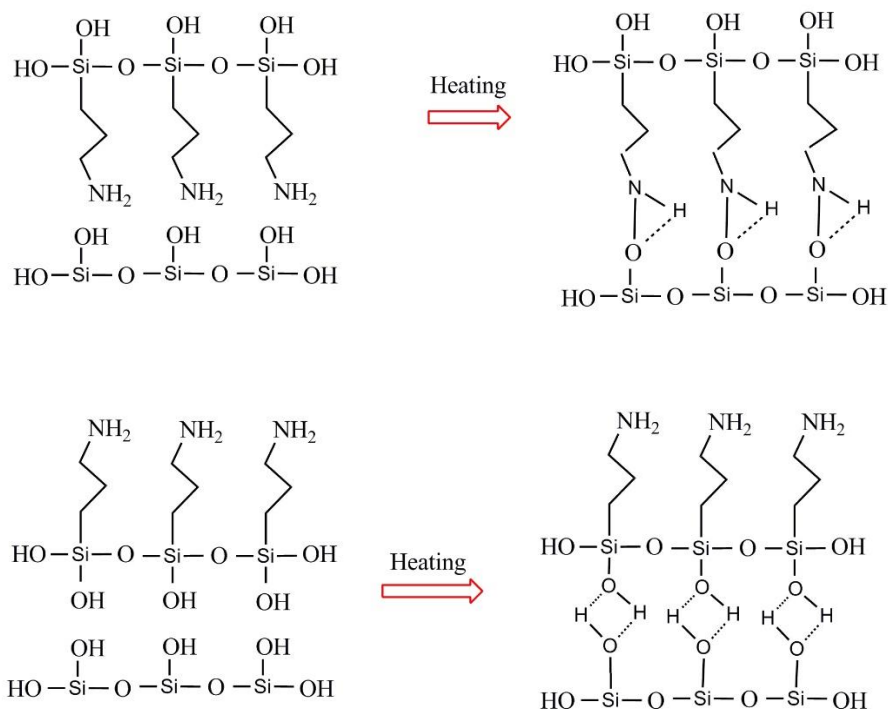
Figure 10 Two possibilities reaction between molecules of APTMS and silica nanoparticles.
