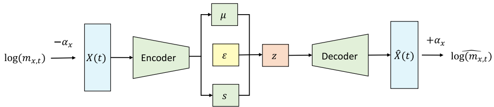
Figure 6. VAE probabilistic reconstruction. The encoder transforms X(t) into a latent probabilistic space with mean \mu and scale s , from which z is sampled by using noise \epsilon . The decoder then reconstructs \hat{X}(t) from z (Miyata & Matsuyama, 2022).
