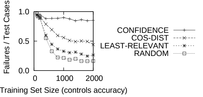
Fig. 6. After removing items that might expose “the same fault” (by distance), CONFIDENCE and COS-DIST approaches still performed very well.
