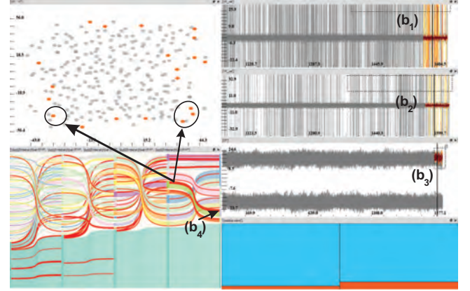
Figure 11: Discovery of jumpers within existing clusterings. The composed brush b_L = (b_1 \cup b_2) \cap b_3 selects the jumpers that are displayed in the animated scatter plot. The cluster view depicts their occurrence in individual clusterings. The cluster containing 4 jumpers was selected ( b_L \cap b_4 ) to reveal their position (arrows and circles) within the cluster. The histogram depicts classification of the jumpers into DMPC and DMPG classes.
