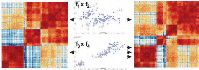
Figure 3: The dissimilarity matrix with the equal weights w_{f_1} = w_{f_2} = w_{f_3} = w_{f_4} = 1 (left). To emphasize the contribution of f_3 and f_4 variables, we tripled (triple arrow) the weights of f_3 and f_4 ; i.e., w_{f_3} = w_{f_4} = 3 (right). For better understanding the corresponding scatterplots for both variable combinations are shown in the middle.
