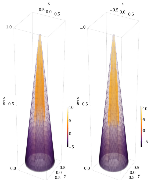
FIG. 5. Logarithm of the LFIE [Eq. (20)] in the region 0.5R(z) < r < 1.5R(z) around the surface of the cone, for material parameters \beta = 16 , \epsilon_w = 25 , and frequency \omega = 0.75\omega_p . Lengths are in units of c/\omega_p . Left: m = -1 and right m = -2 .
