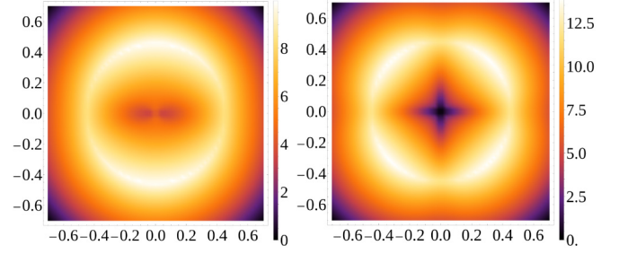
FIG. 6. Illustration of the radial profile of the SPP modes. Here, the logarithm of the LFIE [Eq. (20)] is shown, with parameters \beta = 16 , \epsilon_w = 25 , and \omega = 0.75\omega_p and m = -1 (left) and m = -2 (right). On the axes, the x and y coordinates are in units of c/\omega_p .
