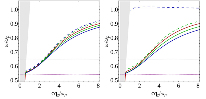
FIG. 2. Size dependence of the SPP dispersion relation in a cylindrical WS waveguide. The parameters were chosen as \beta = 16 , \epsilon_W = 25 , \epsilon_d = 1 , and \rho = 4 (left) and \rho = 2.4 (right). Here, we show the bands m = 0 (solid red), m = 1 (dashed green), m = -1 (solid green), m = 2 (dashed blue), and m = -2 (solid blue). The dotted purple line is the frequency \omega_- [see Eq. (13)]. The dotted black line denotes a given frequency, here \omega = 0.65\omega_p . For the larger section, the waveguide supports the m = 2 mode at that frequency, while for the smaller one, this mode is not supported.
