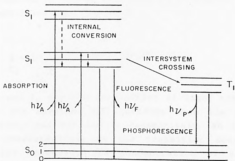
Figure A2.2 - Jablonski diagram
