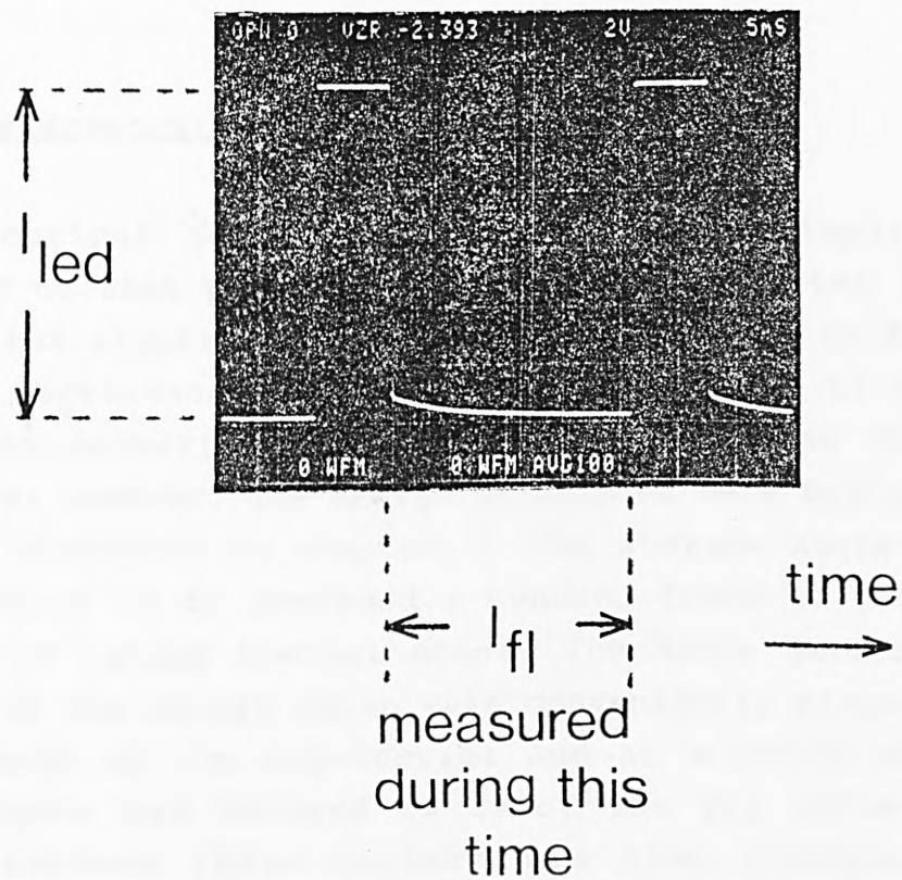
Figure 4.5 - Photograph of detected signal showing 'probe' signal I_{led} and fluorescence emission I_{fl}
