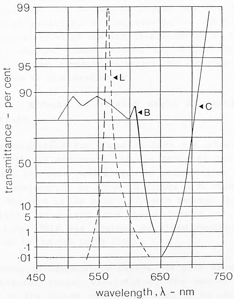
Figure 6.7 - Transmission characteristics.
