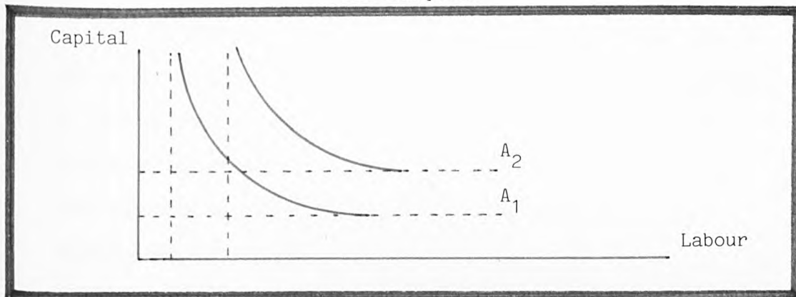
figure 4.12 The Isoquant
