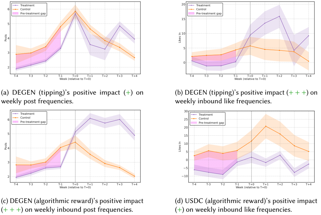
Fig. 5. Difference-in-Differences (DID) visualizations.
