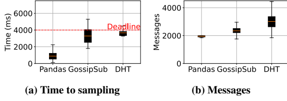
Figure 12: Distribution of time to sampling and messages compared to baselines based on GossipSub and the Kademlia DHT.
