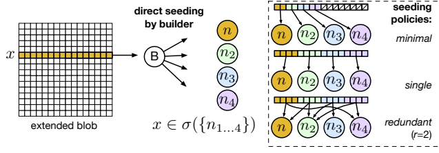
Figure 6: Three seeding policies. The “minimal” policy splits the first half of each row or column amongst known peers having it in their assignment. The “single” policy splits the entire row or column. The “redundant” policy shares each split to r nodes.
