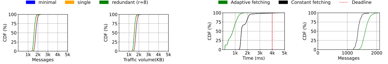
Figure 10: Distribution of messages and traffic volume for fetch across nodes, for different seeding strategies.
