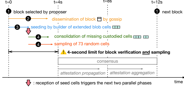
Figure 5: Timeline of events within a slot. Starting from the selection of a new block by the proposer (time 0, ❶), two concurrent processes start for nodes that must both terminate within 4 seconds: block dissemination (❷) and extended blob data dissemination (❸), consolidation, and sampling (❹).
