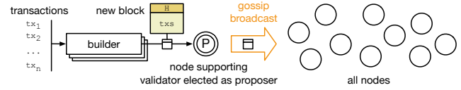
Figure 1: Proposer-Builder Separation (PBS). The proposer, elected based on stake, selects a block among those prepared by builders. The block is broadcast by gossip to all nodes.
