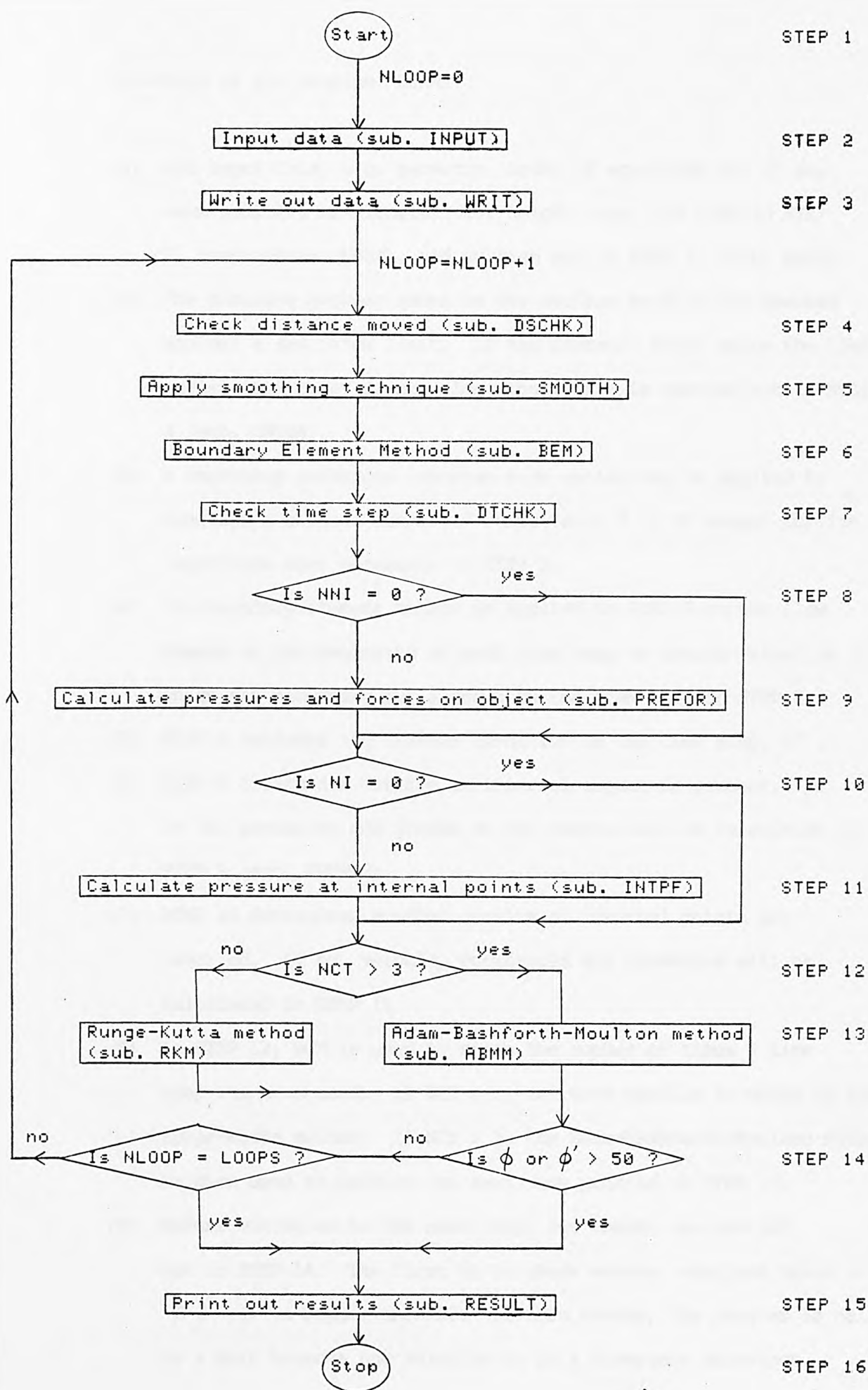
Fig. 6.2.1 Simplified flow chart for 'BEMW1'
