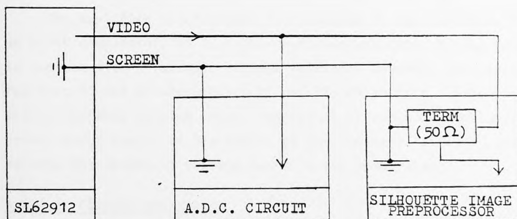
Figure A.5: Connection of video signal
