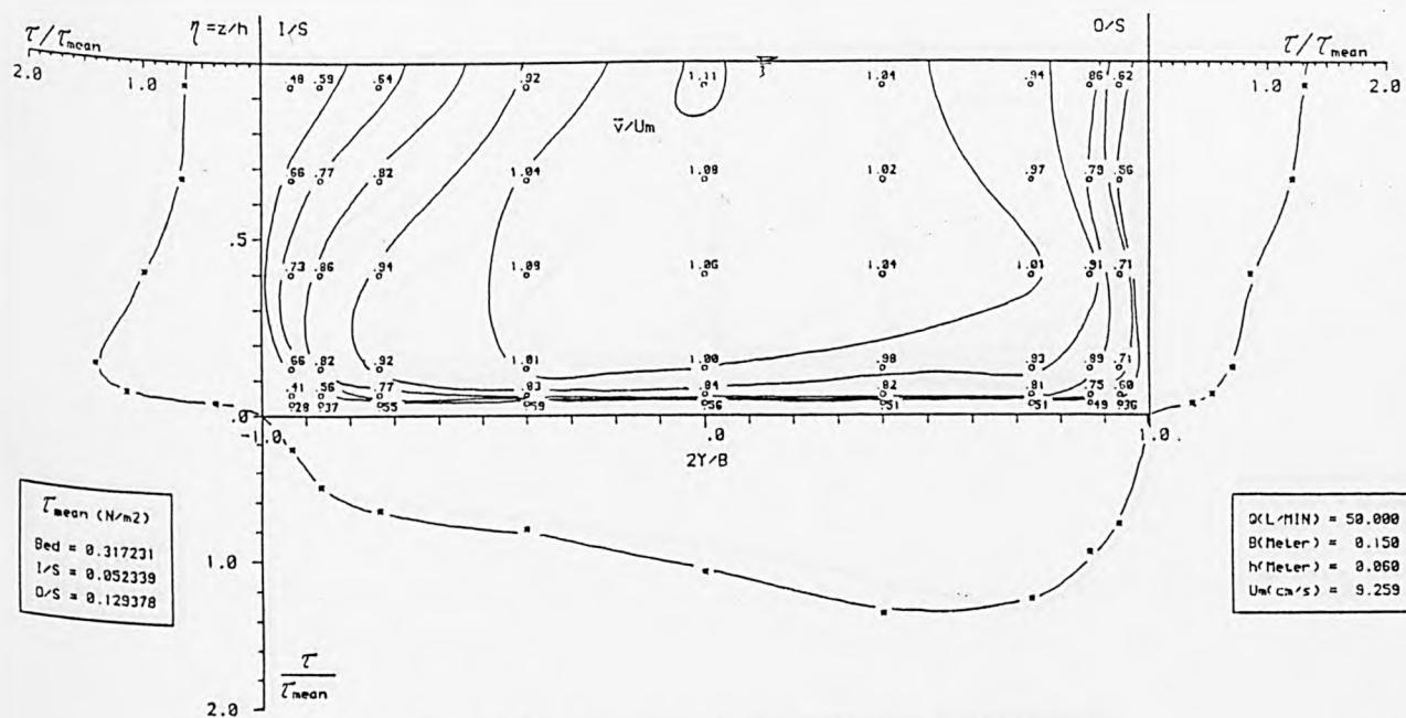
Fig. 6.93 Isovels of the velocity distribution in the direction of flow and boundary shear stress at section U-2, run no.3
