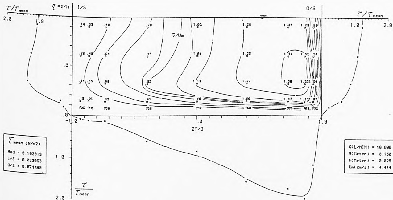
Fig. 6.106 Isovels of the velocity distribution in the direction of flow and boundary shear stress at section S-3, run no.1
