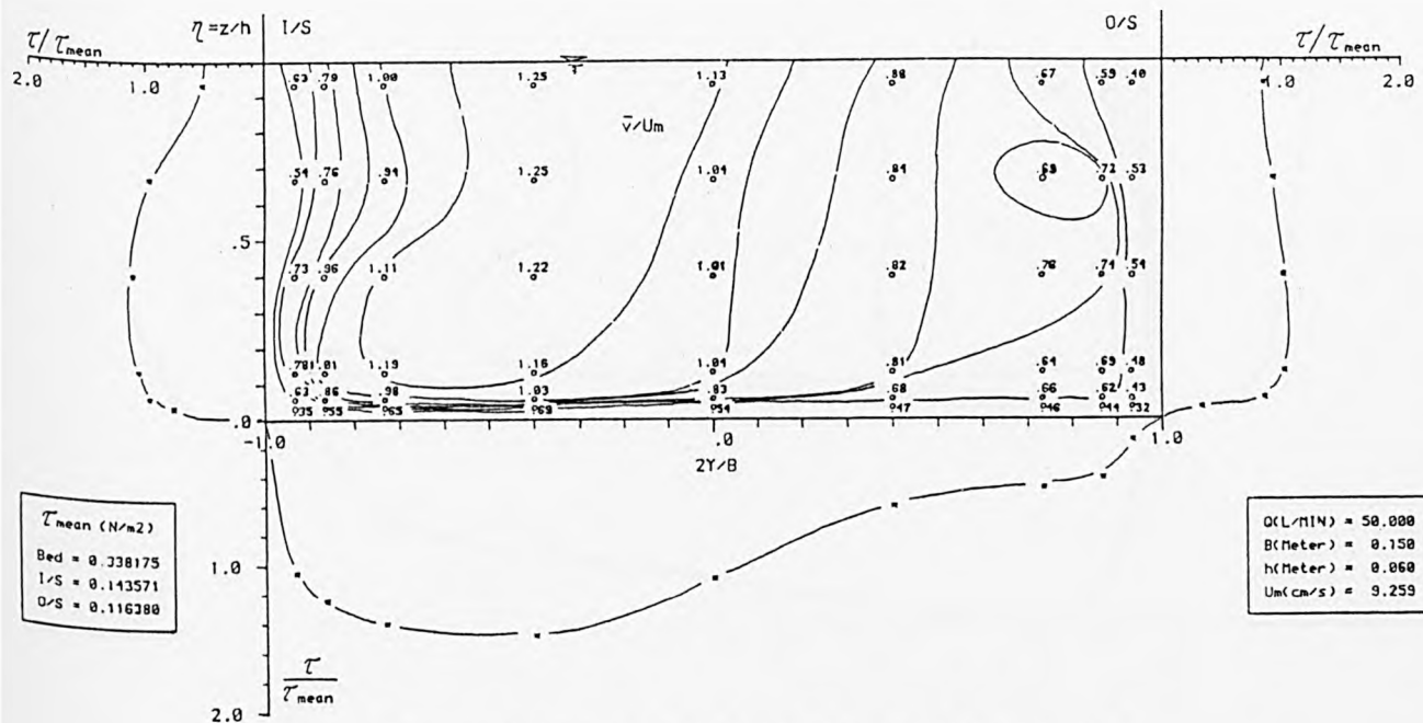
Fig. 6.117 Isovels of the velocity distribution in the direction of flow and boundary shear stress at section S-6, run no.3
