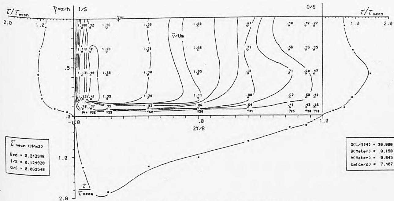
Fig. 6.113 Isovels of the velocity distribution in the direction of flow and boundary shear stress at section S-5, run no.2
