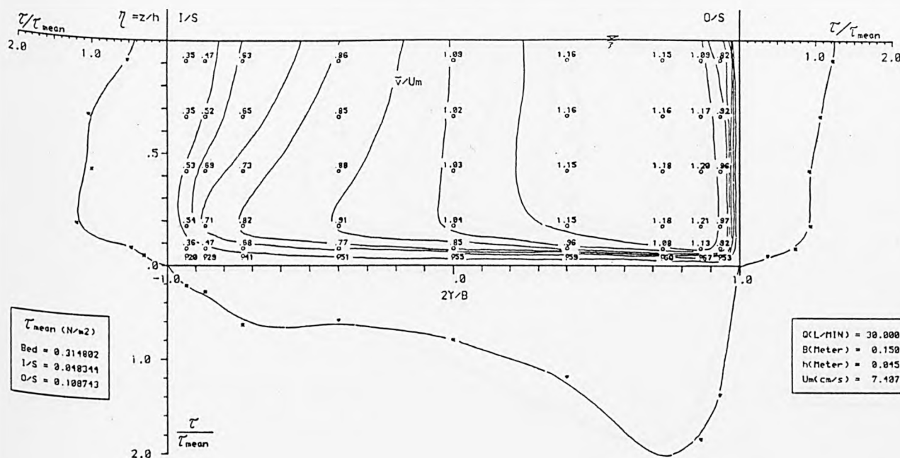
Fig. 6.107 Isovels of the velocity distribution in the direction of flow and boundary shear stress at section S-3, run no.2
