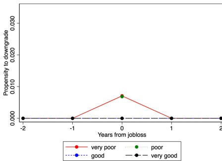
FIGURE 10. Simulated downgrading by car quality. Note: There are 4 levels of quality: very poor (quality less than 90% of average among sold cars), poor (between 90% and 100%), good (100% to 110%), and very good (over 110% of average).
