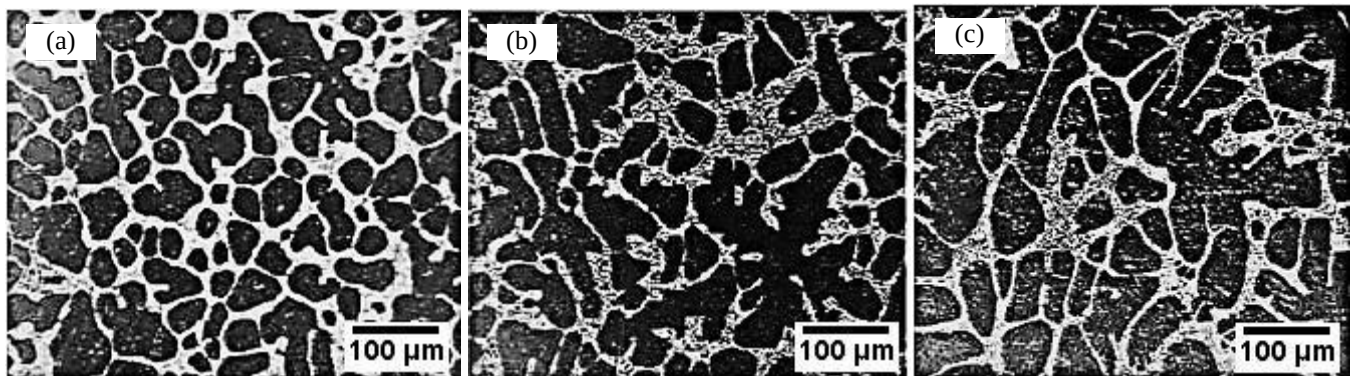
FIGURE 4. - Microstructures from a 45s holding time and with pouring temperatures of (a) 630°C, (b) 650°C and (c) 680°C.
