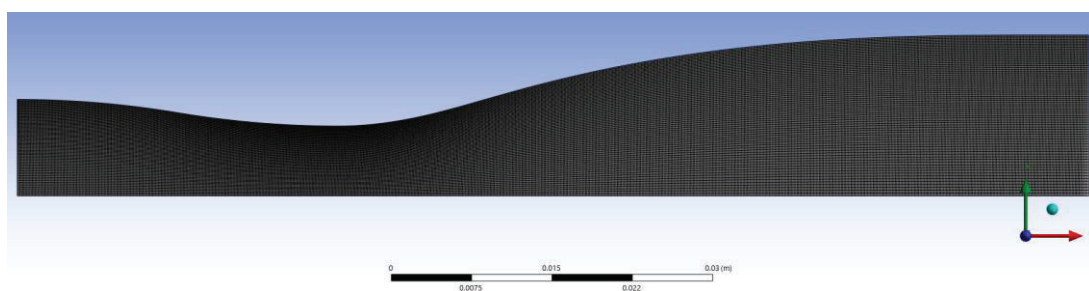
Figure 2: Medium mesh used for the inviscid 2D CFD simulations.
