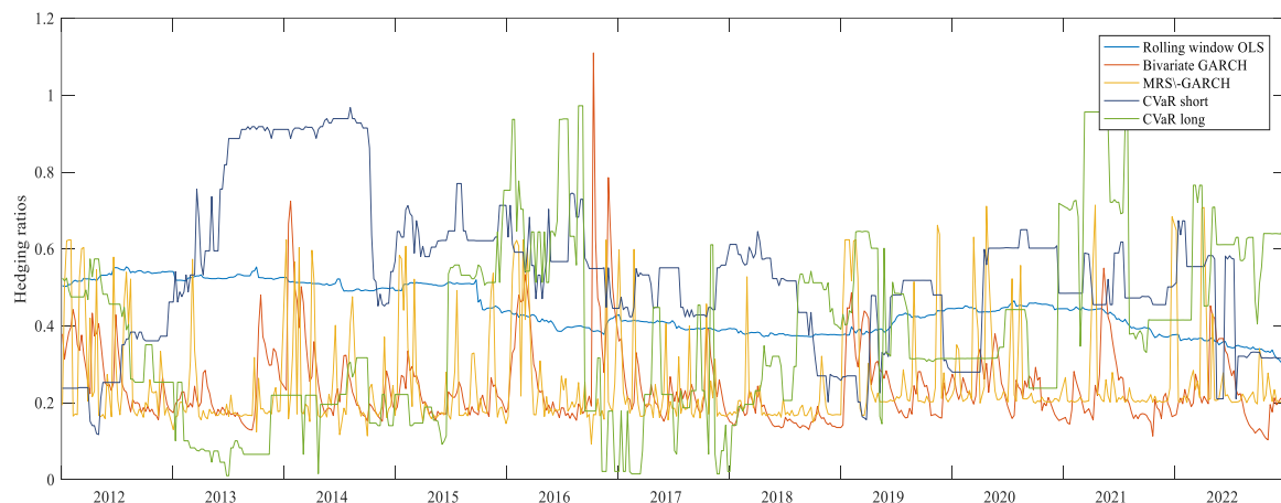
Fig. 5. Estimates of out-of-sample dynamic hedging ratios for Supramax
