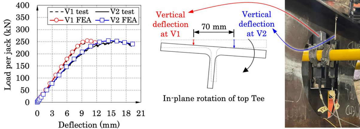
Figure 7. Test results and FEA validation showing rotation of the top Tee at centreline of the opening.
