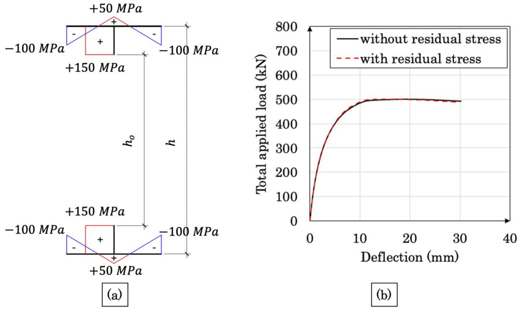
Figure 6. Residual stresses: (a) pattern for cellular beams based on Sonck [12], (b) comparison of load-displacement curves for the case of h_o = 425 mm, s_o = 180 mm, t_w = 7 mm, and S355 steel, with and without residual stresses.
