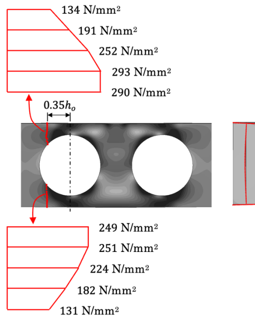
Figure 14. Average Von Mises stress in Tees at onset of web-post buckling ( F_{w.FEA} = 364 kN, LPF = 0.74) (the case of h_o = 400\text{mm} , s_o = 205\text{mm} , t_w = 9\text{mm} , and S355 steel).
