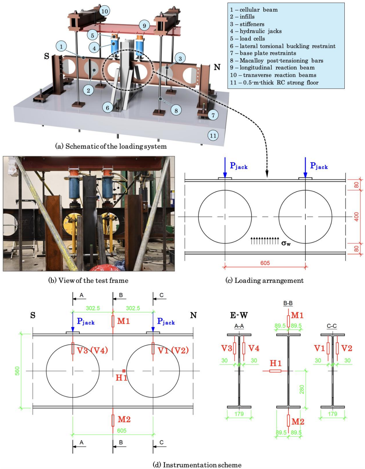
Figure 2. Details of the test setup (units: millimetres).
