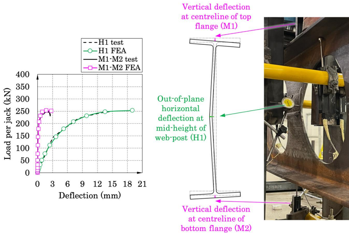
Figure 8. Test results and FEA validation showing vertical shortening (M1-M2) and horizontal deflection (H1) at centreline of the web-post.
