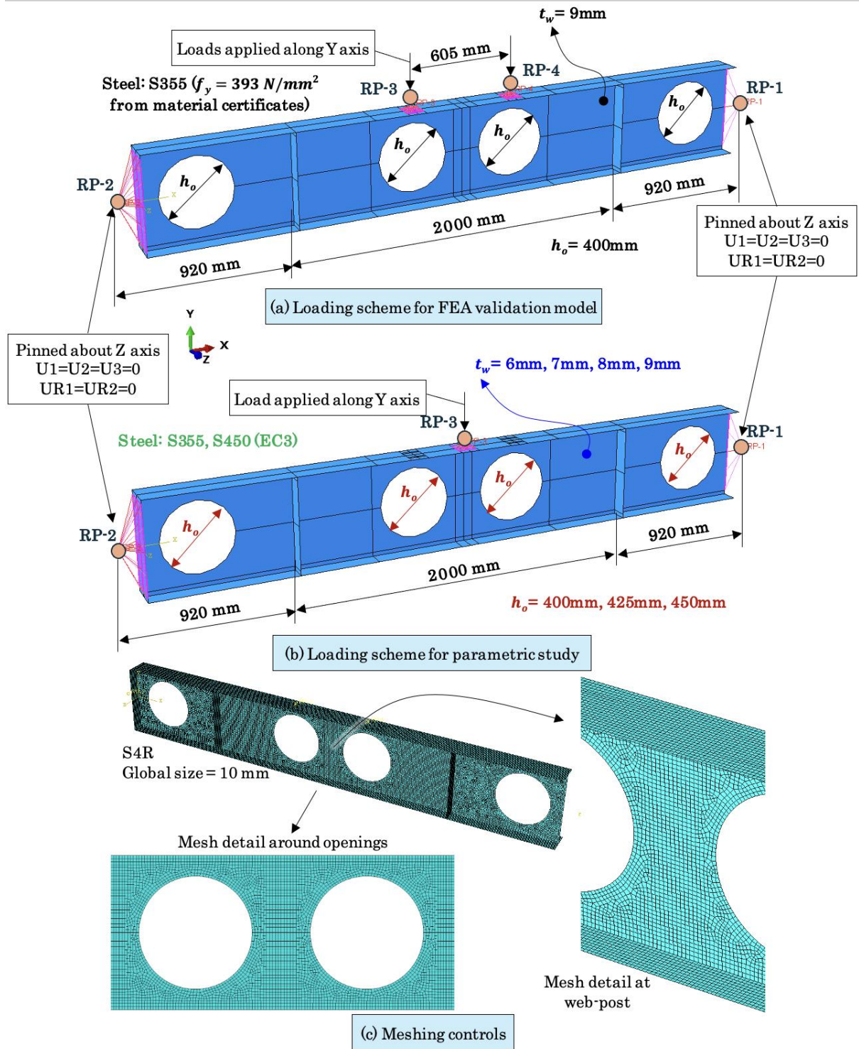
Figure 3. Details of the FE models of the cellular beams.
