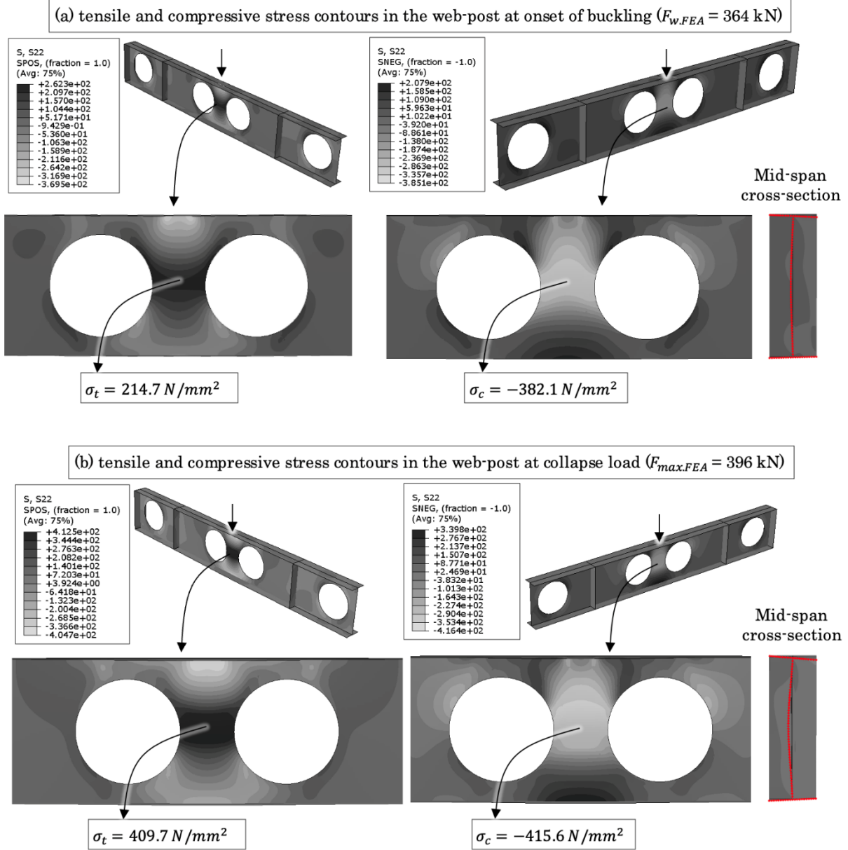
Figure 10. Vertical stress contours in the web-post (the case of h_o = 400\text{mm} , s_o = 205\text{mm} , t_w = 9\text{mm} , and S355 steel).
