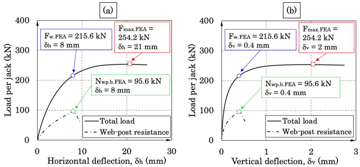
Figure 9. Analysis of loading versus displacement curves from FEA model of the test.
