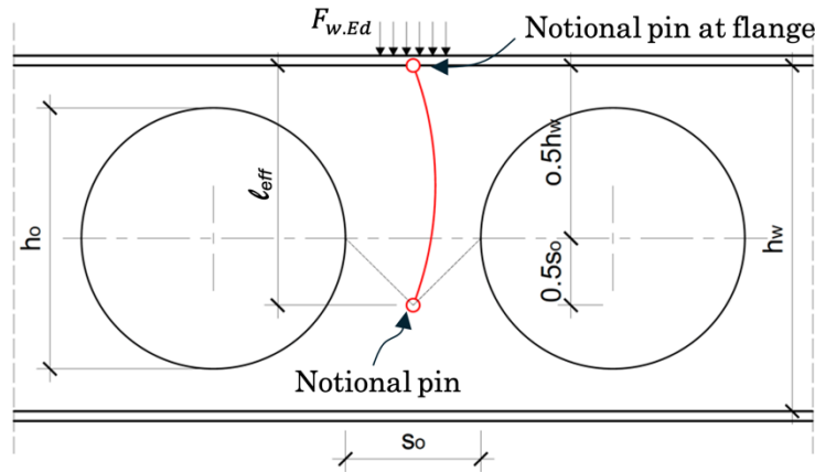
Figure 13. Mechanical model showing proposed effective length for web-post buckling using equivalent strut buckling method to BS EN 1993-1-1.
