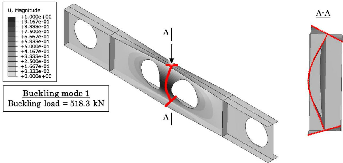
Figure 5. Buckling modes for the case of a single point load (in which the buckling load is the load corresponding to the load point and deformation scale factor = 100).
