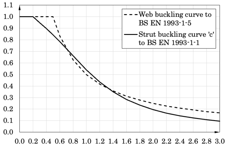
Figure 1. Comparison between plate buckling and strut buckling curve “c” for various web slenderness ratios.
