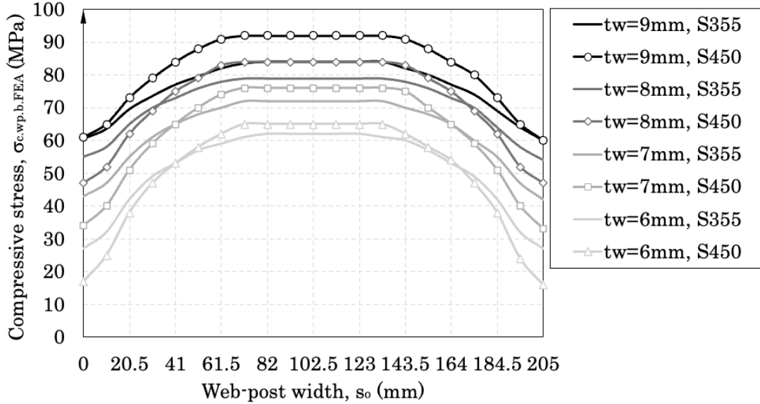
Figure 11. Compressive stress profiles across the web-post width obtained from the FEA (for h_o = 400\text{mm} and s_o = 205\text{mm} ).
