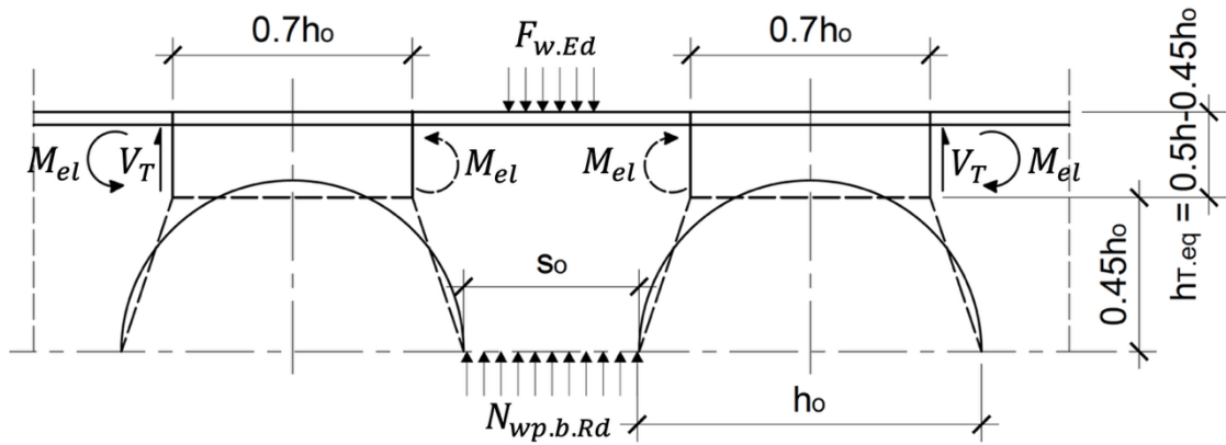
Figure 15. Equilibrium of forces on web-post including Vierendeel bending of the top Tees.
