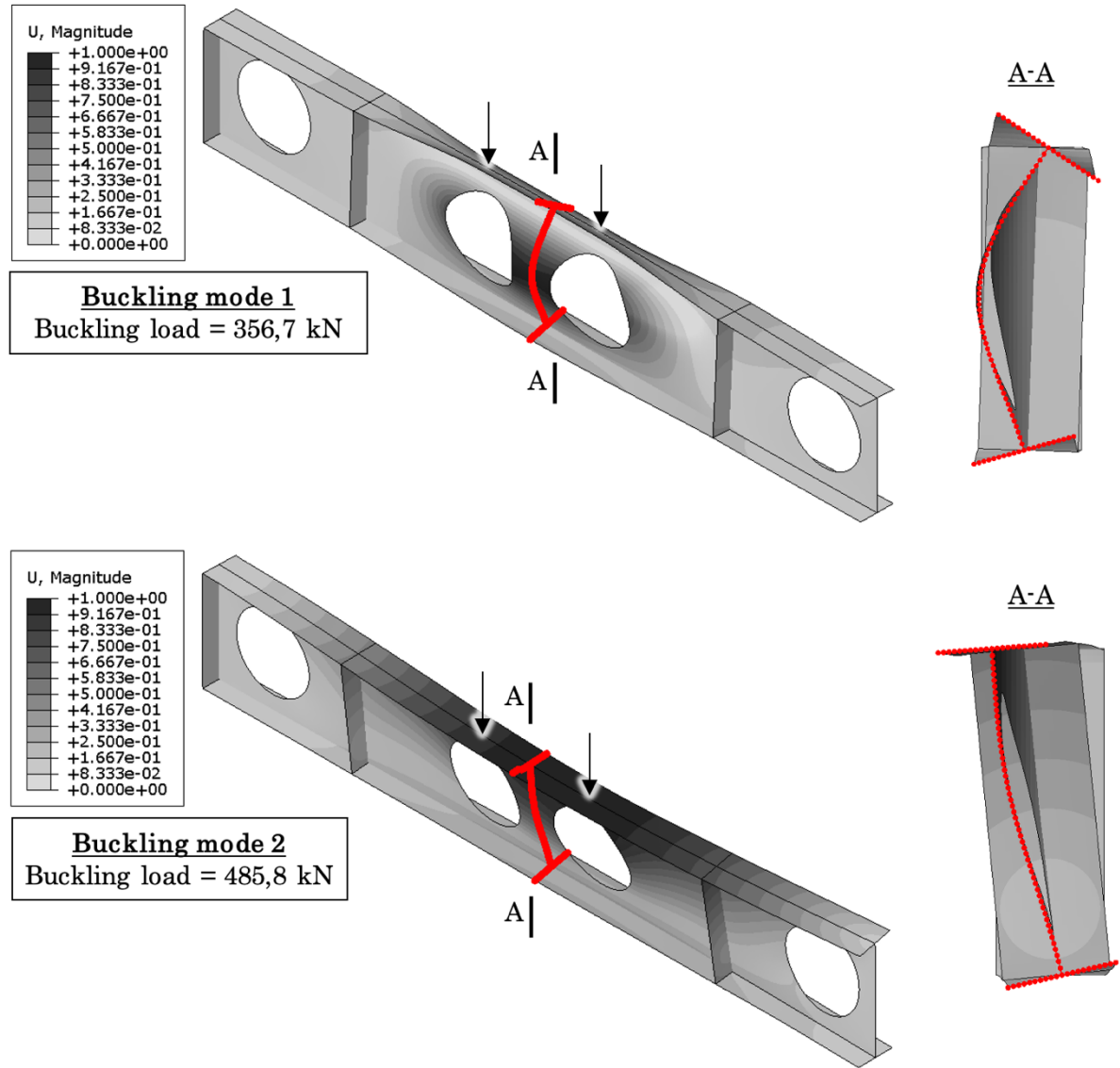
Figure 4. Buckling modes for the test arrangement (in which the buckling load is the load corresponding to each load point and deformation scale factor = 100).
