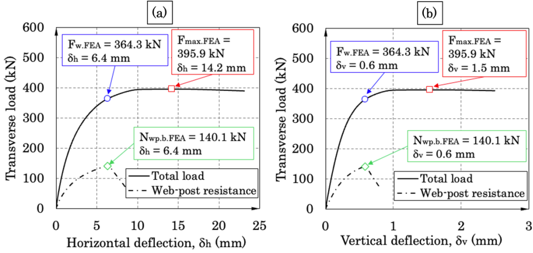
Figure 12. Loading vs. displacement curves from FEA (the case of h_o = 400\text{mm} , s_o = 205\text{mm} , t_w = 9\text{mm} , and S355 steel).
