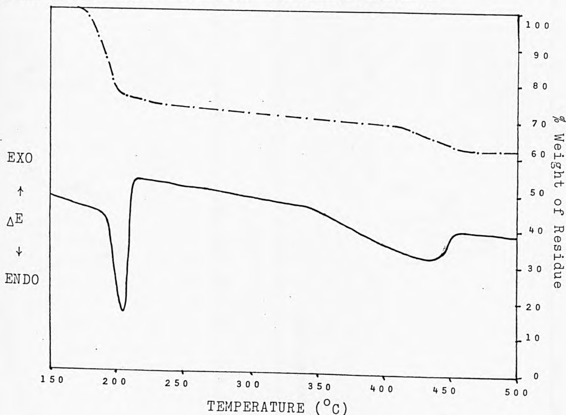
Figure 3.25. TG/DTA Trace for \text{K}_2\text{Sn}_2(\text{CH}_2\text{C}_2\text{O}_4)_3\cdot\text{H}_2\text{O}
