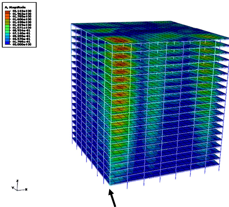
Fig. 16 Acceleration contour of Case 2
