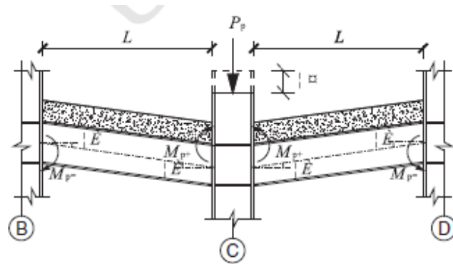
Fig. 10. Plastic hinge action.
