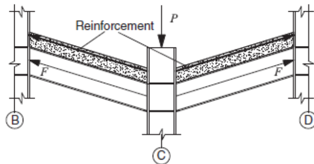
Fig. 11. Catenary action.
