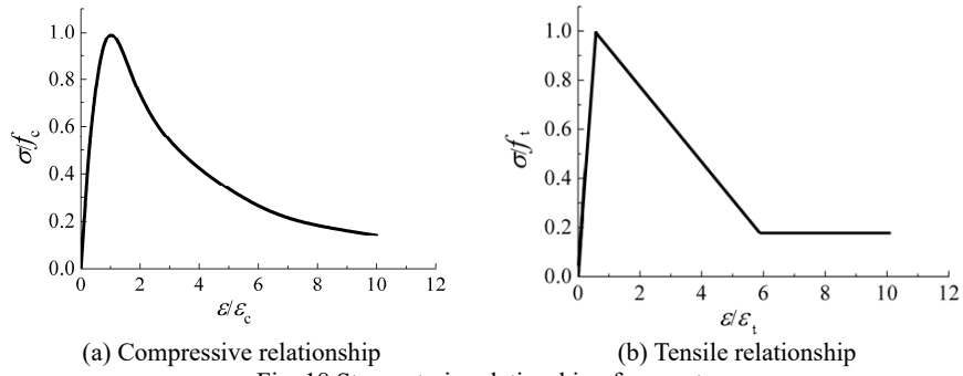
Fig. 18 Stress-strain relationship of concrete
