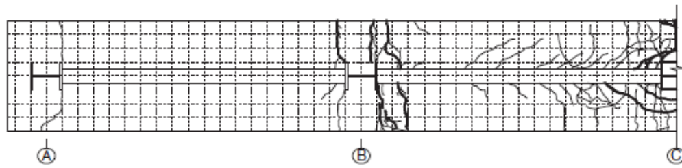
b) Crack distribution on the bottom surface of RC slab
