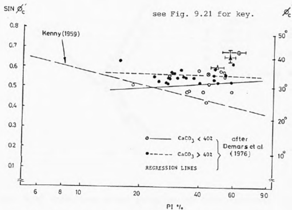
Fig. 9.22 Relationship between \text{SIN } \phi'_c and Plasticity Index
