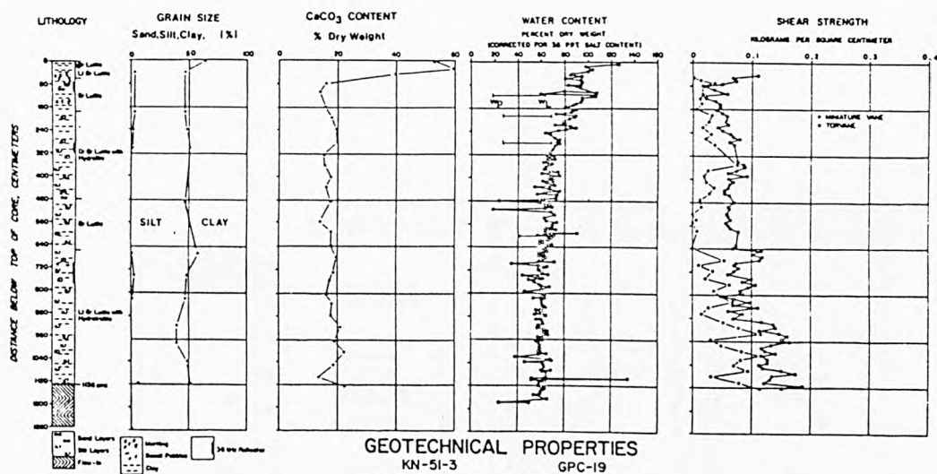
Fig. 4.7 Geotechnical Properties ( KNORR-51 )
