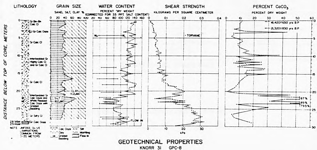
Fig. 4.6 Geotechnical Properties ( KNORR-31 , North Atlantic )
