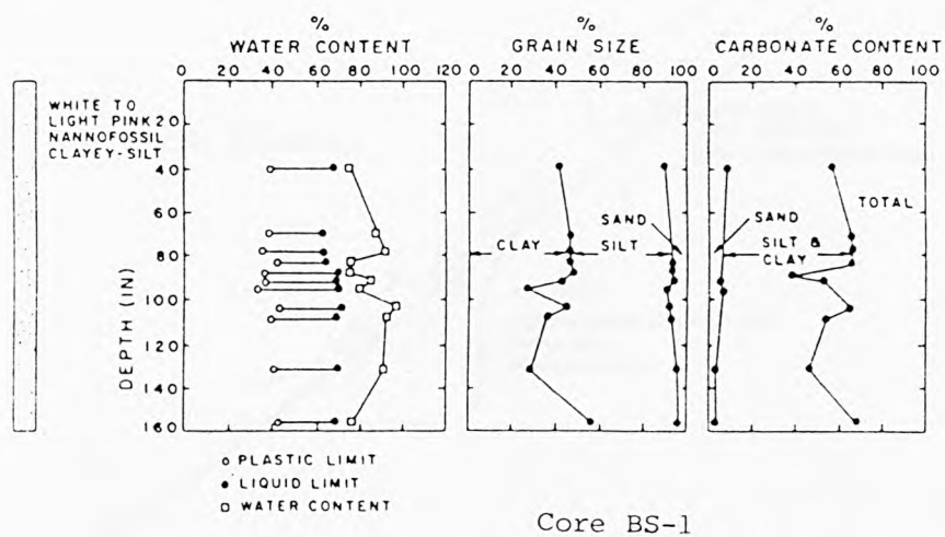
Fig. 4.10 Geotechnical Properties (North Atlantic, after Demars, 1975 )
