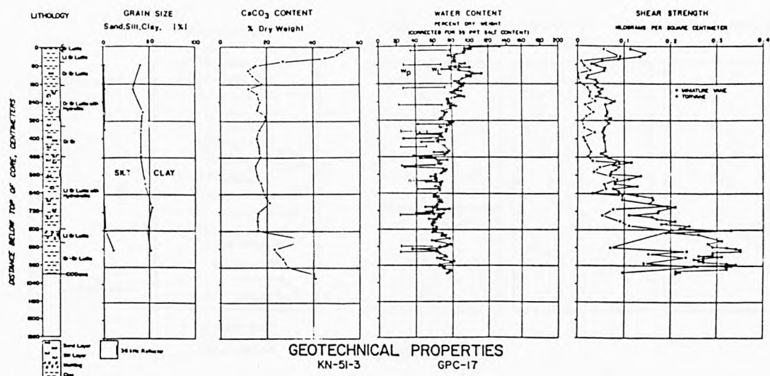
Fig. 4.7 Geotechnical Properties ( KNORR-51 )
