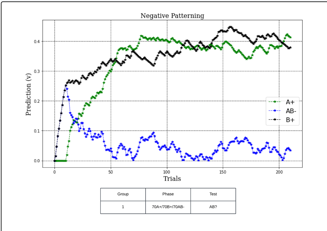
Figure 5.15: Negative patterning results demonstrating successful non-linear discrimination. The learning curves reveal a complex pattern that cannot be explained by simple elemental summation. Both A (green line) and B (black line) acquire positive associative strength ( V \sim 0.41 ). Critically, the compound AB (blue line) shows different learning dynamics: after initial exploration, it maintains near-zero values around V \sim 0.05 . The separation between element and compound values demonstrates the model's ability to treat AB as a unique configuration rather than the sum of its parts. If the model operated purely on elemental summation, AB should have V \sim 0.82 (sum of A and B); instead, it maintains near-zero associative strength, confirming successful negative patterning discrimination.
